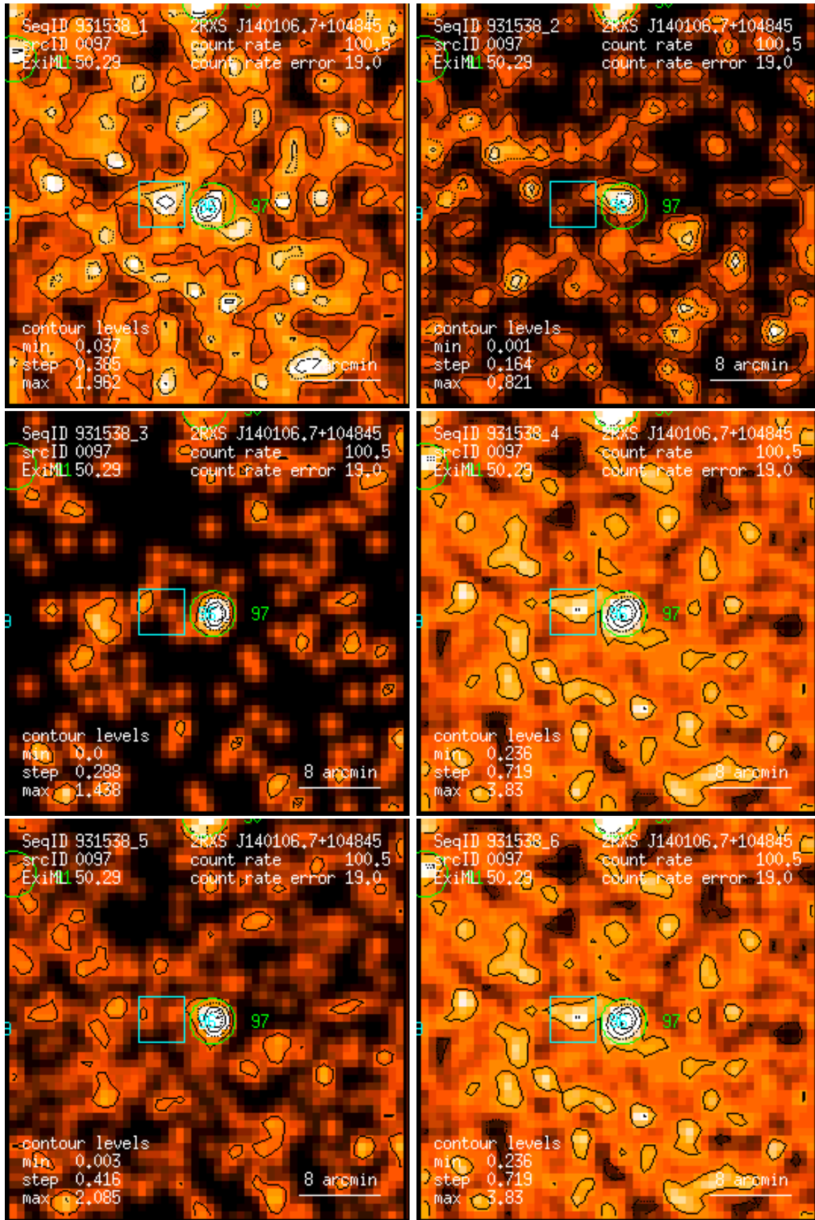
Figure 97: RASS 931538: detection 0097: band rate images, Gaussian filter: (1) PSPC channels 11 – 41, (2) 52 – 90, (3) 91 – 201, (4) 11 – 235, (5) 52 – 201, (6) 11 – 201. Broad band rates in counts/ks. Band rate contour levels in counts/ks/arcmin 2 .
