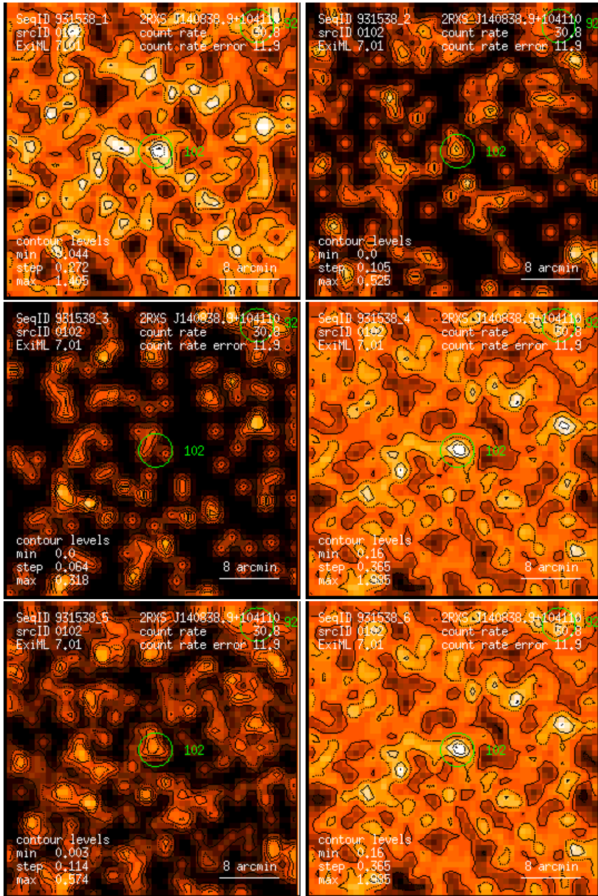
Figure 102: RASS 931538: detection 0102: band rate images, Gaussian filter: (1) PSPC channels 11 – 41, (2) 52 – 90, (3) 91 – 201, (4) 11 – 235, (5) 52 – 201, (6) 11 – 201. Broad band rates in counts/ks. Band rate contour levels in counts/ks/arcmin 2 .
