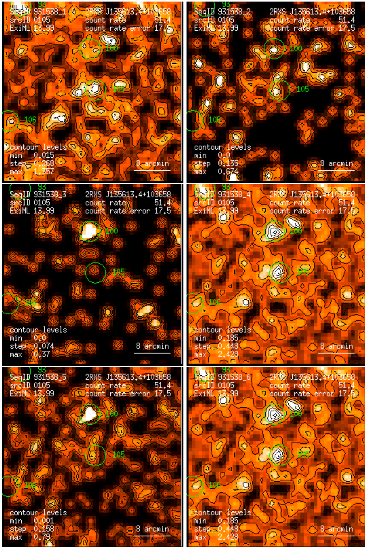
Figure 105: RASS 931538: detection 0105: band rate images, Gaussian filter: (1) PSPC channels 11 – 41, (2) 52 – 90, (3) 91 – 201, (4) 11 – 235, (5) 52 – 201, (6) 11 – 201. Broad band rates in counts/ks. Band rate contour levels in counts/ks/arcmin 2 .
