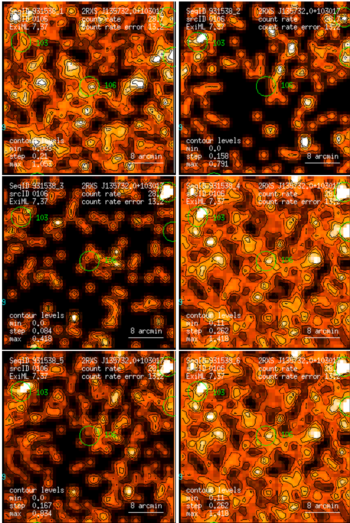
Figure 106: RASS 931538: detection 0106: band rate images, Gaussian filter: (1) PSPC channels 11 – 41, (2) 52 – 90, (3) 91 – 201, (4) 11 – 235, (5) 52 – 201, (6) 11 – 201. Broad band rates in counts/ks. Band rate contour levels in counts/ks/arcmin 2 .
