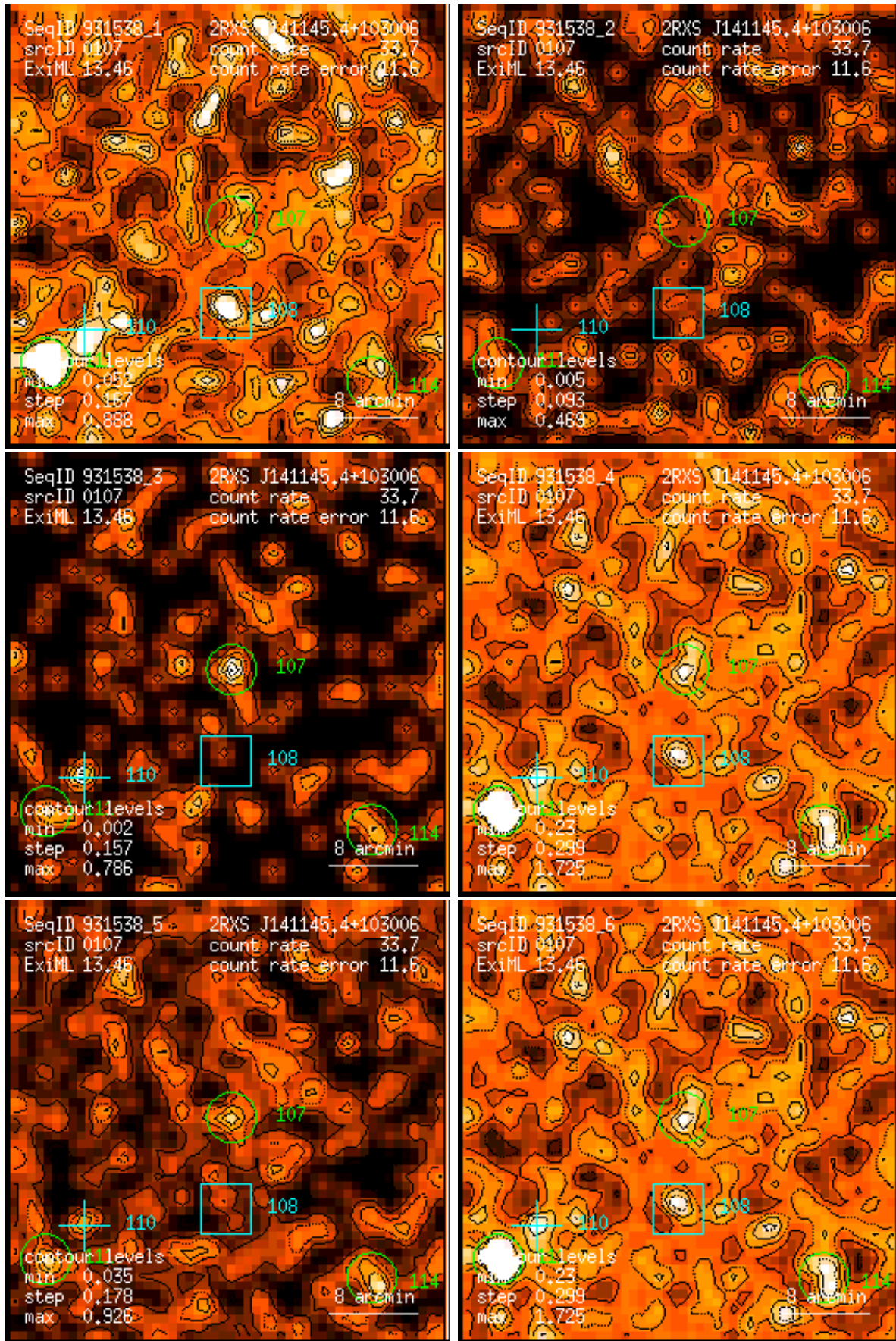
Figure 107: RASS 931538: detection 0107: band rate images, Gaussian filter: (1) PSPC channels 11 – 41, (2) 52 – 90, (3) 91 – 201, (4) 11 – 235, (5) 52 – 201, (6) 11 – 201. Broad band rates in counts/ks. Band rate contour levels in counts/ks/arcmin 2 .
