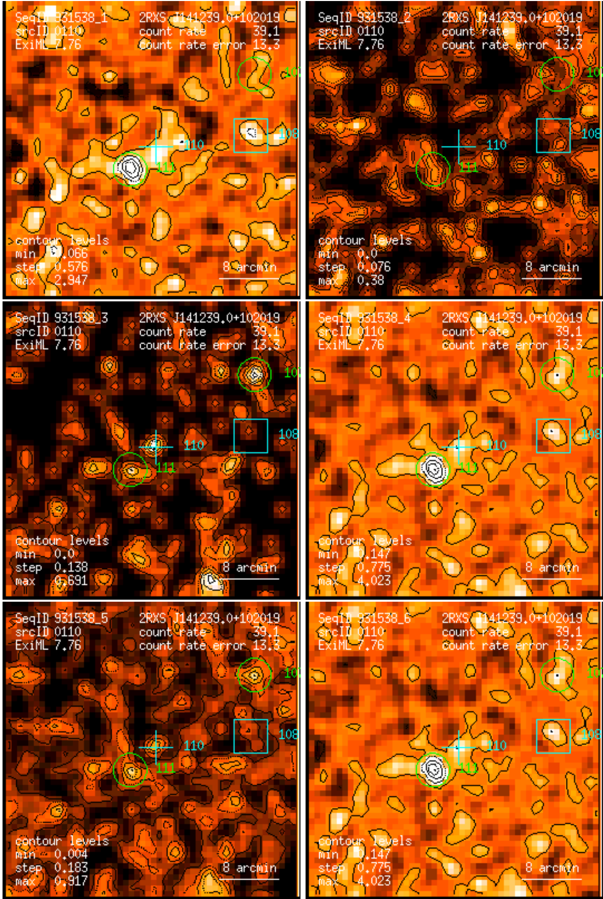
Figure 110: RASS 931538: detection 0110: band rate images, Gaussian filter: (1) PSPC channels 11 – 41, (2) 52 – 90, (3) 91 – 201, (4) 11 – 235, (5) 52 – 201, (6) 11 – 201. Broad band rates in counts/ks. Band rate contour levels in counts/ks/arcmin 2 .
