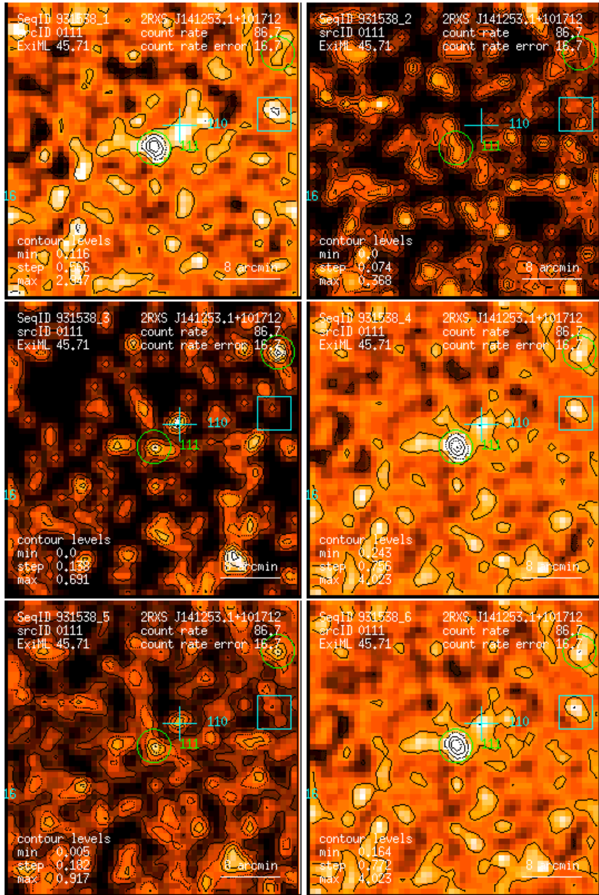
Figure 111: RASS 931538: detection 0111: band rate images, Gaussian filter: (1) PSPC channels 11 – 41, (2) 52 – 90, (3) 91 – 201, (4) 11 – 235, (5) 52 – 201, (6) 11 – 201. Broad band rates in counts/ks. Band rate contour levels in counts/ks/arcmin 2 .
