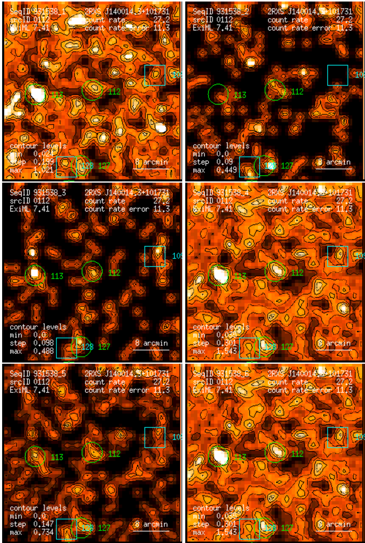
Figure 112: RASS 931538: detection 0112: band rate images, Gaussian filter: (1) PSPC channels 11 – 41, (2) 52 – 90, (3) 91 – 201, (4) 11 – 235, (5) 52 – 201, (6) 11 – 201. Broad band rates in counts/ks. Band rate contour levels in counts/ks/arcmin 2 .
