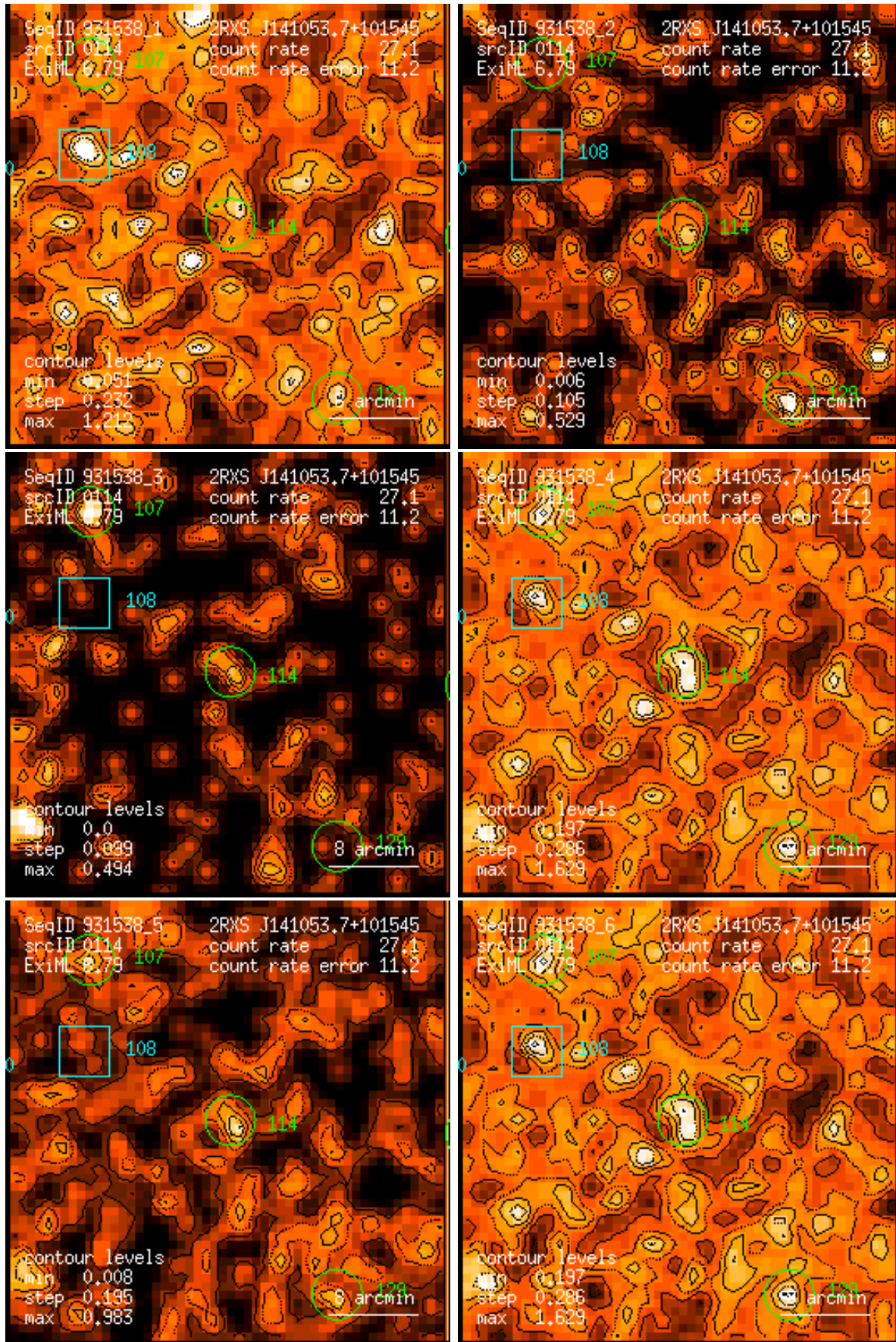
Figure 114: RASS 931538: detection 0114: band rate images, Gaussian filter: (1) PSPC channels 11 – 41, (2) 52 – 90, (3) 91 – 201, (4) 11 – 235, (5) 52 – 201, (6) 11 – 201. Broad band rates in counts/ks. Band rate contour levels in counts/ks/arcmin 2 .
