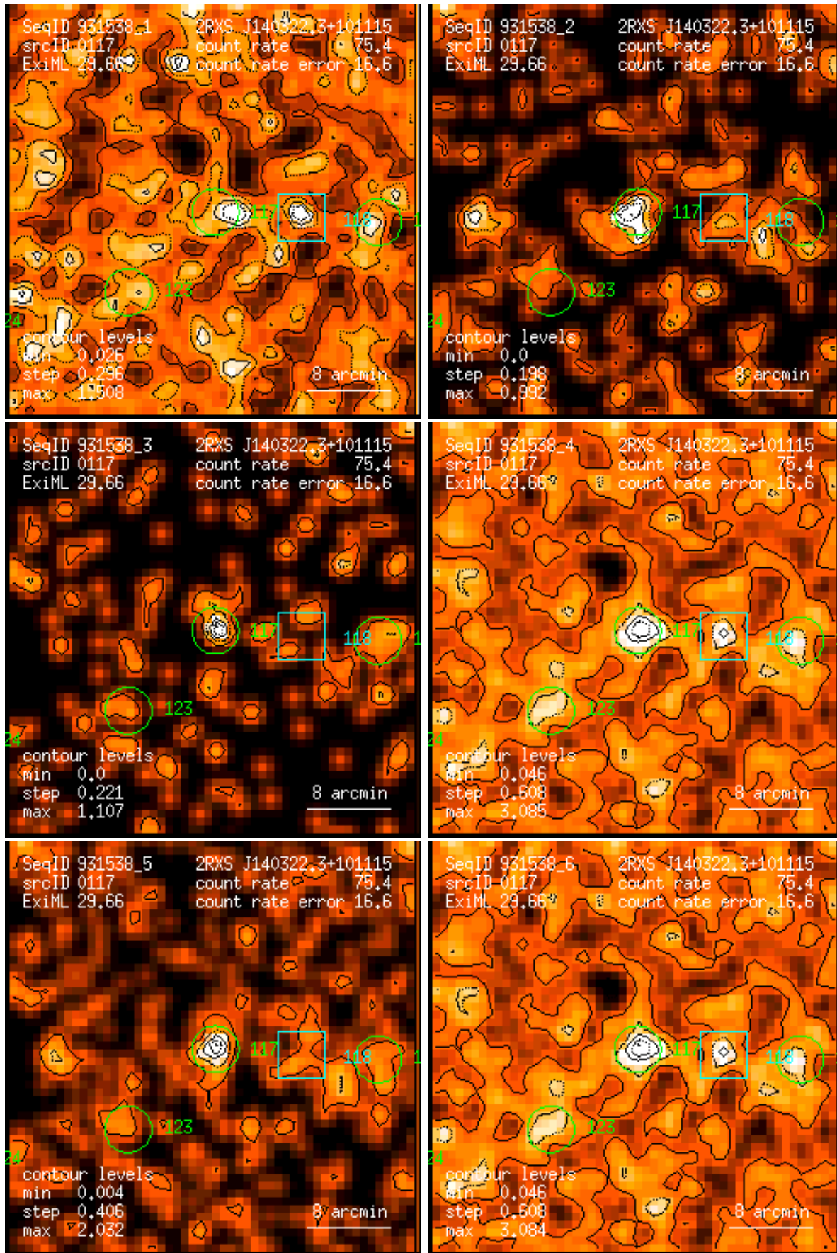
Figure 117: RASS 931538: detection 0117: band rate images, Gaussian filter: (1) PSPC channels 11 – 41, (2) 52 – 90, (3) 91 – 201, (4) 11 – 235, (5) 52 – 201, (6) 11 – 201. Broad band rates in counts/ks. Band rate contour levels in counts/ks/arcmin 2 .
