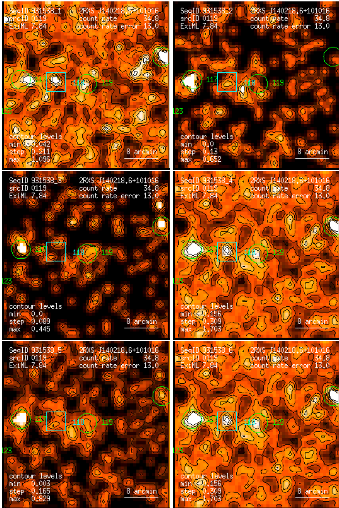
Figure 119: RASS 931538: detection 0119: band rate images, Gaussian filter: (1) PSPC channels 11 – 41, (2) 52 – 90, (3) 91 – 201, (4) 11 – 235, (5) 52 – 201, (6) 11 – 201. Broad band rates in counts/ks. Band rate contour levels in counts/ks/arcmin 2 .
