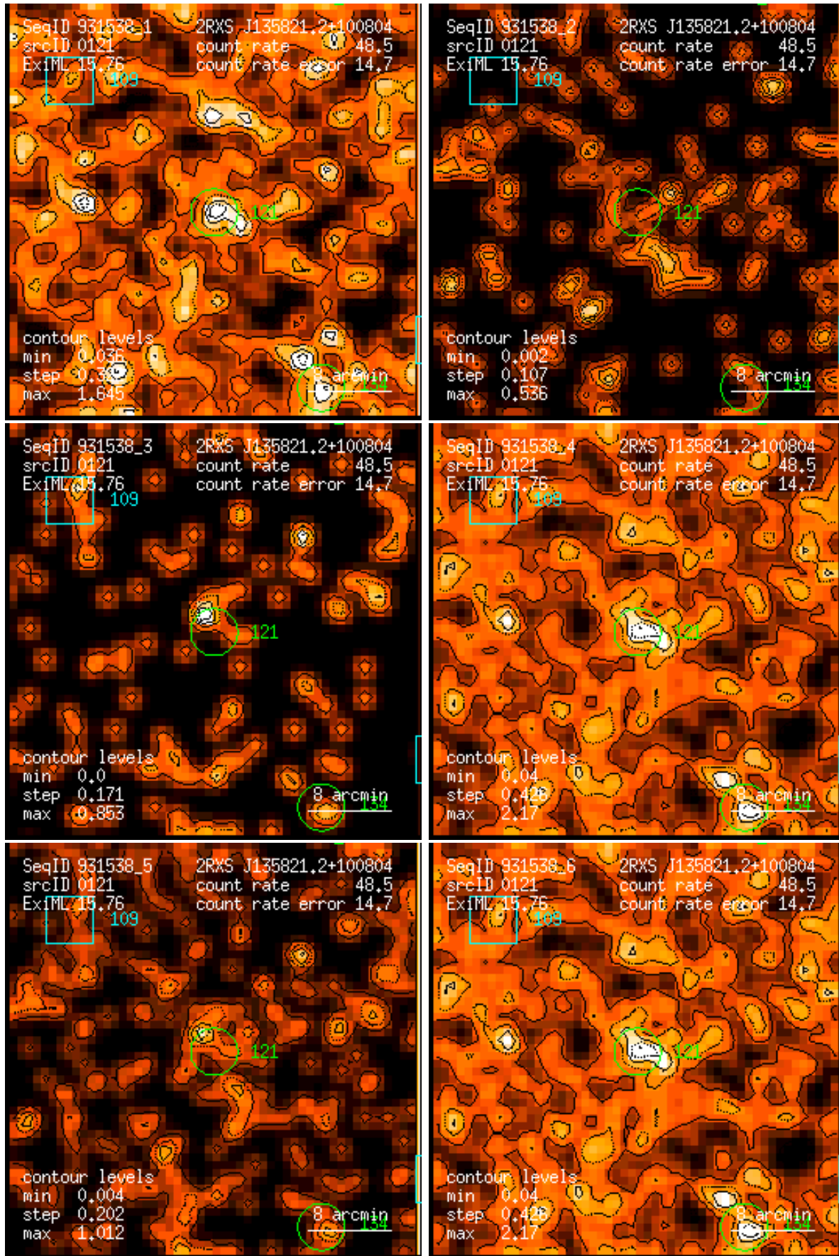
Figure 121: RASS 931538: detection 0121: band rate images, Gaussian filter: (1) PSPC channels 11 – 41, (2) 52 – 90, (3) 91 – 201, (4) 11 – 235, (5) 52 – 201, (6) 11 – 201. Broad band rates in counts/ks. Band rate contour levels in counts/ks/arcmin 2 .
