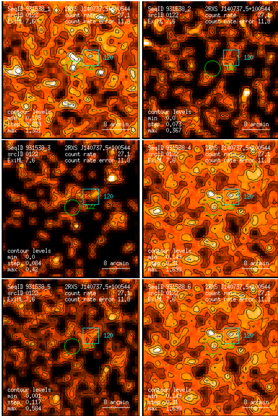
Figure 122: RASS 931538: detection 0122: band rate images, Gaussian filter: (1) PSPC channels 11 – 41, (2) 52 – 90, (3) 91 – 201, (4) 11 – 235, (5) 52 – 201, (6) 11 – 201. Broad band rates in counts/ks. Band rate contour levels in counts/ks/arcmin 2 .
