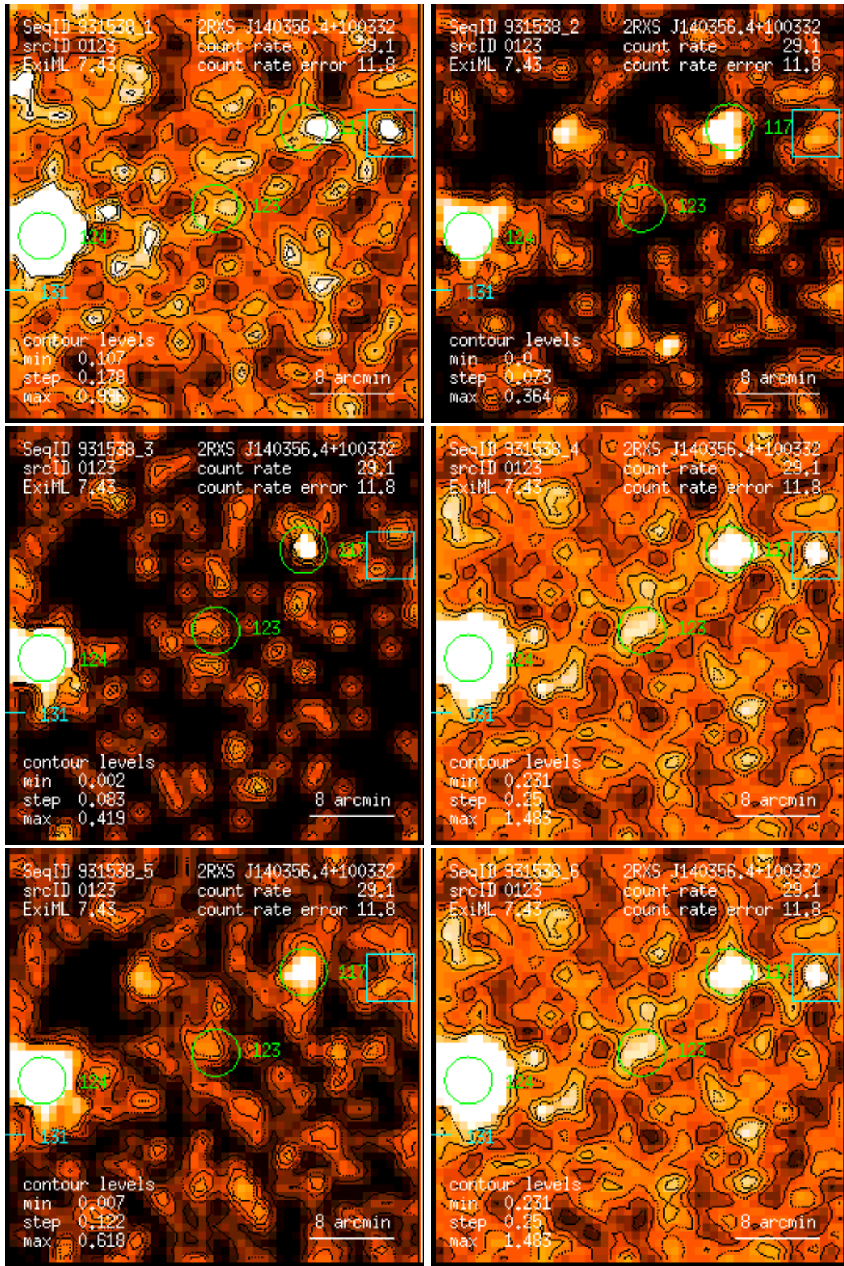
Figure 123: RASS 931538: detection 0123: band rate images, Gaussian filter: (1) PSPC channels 11 – 41, (2) 52 – 90, (3) 91 – 201, (4) 11 – 235, (5) 52 – 201, (6) 11 – 201. Broad band rates in counts/ks. Band rate contour levels in counts/ks/arcmin 2 .
