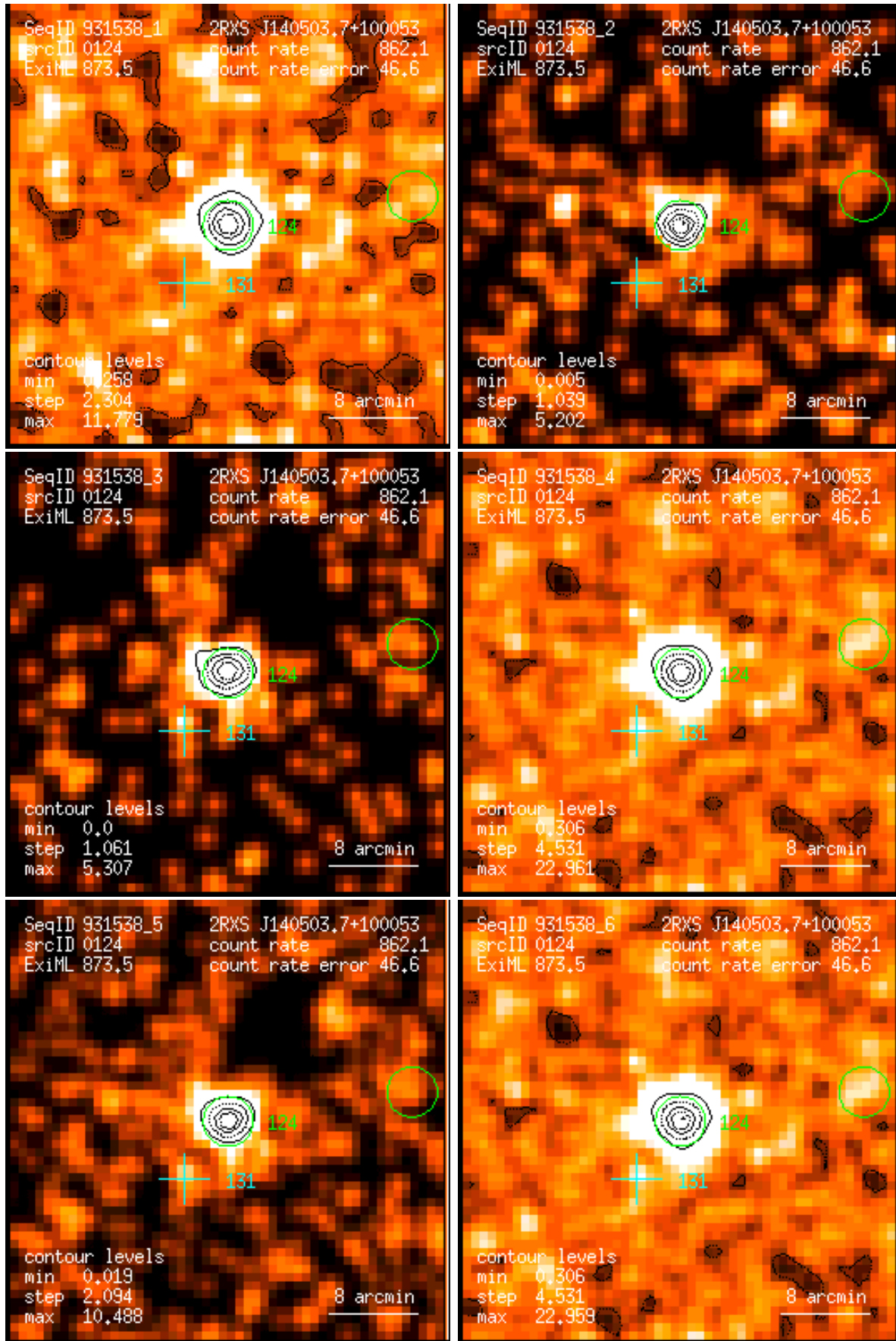
Figure 124: RASS 931538: detection 0124: band rate images, Gaussian filter: (1) PSPC channels 11 – 41, (2) 52 – 90, (3) 91 – 201, (4) 11 – 235, (5) 52 – 201, (6) 11 – 201. Broad band rates in counts/ks. Band rate contour levels in counts/ks/arcmin 2 .
