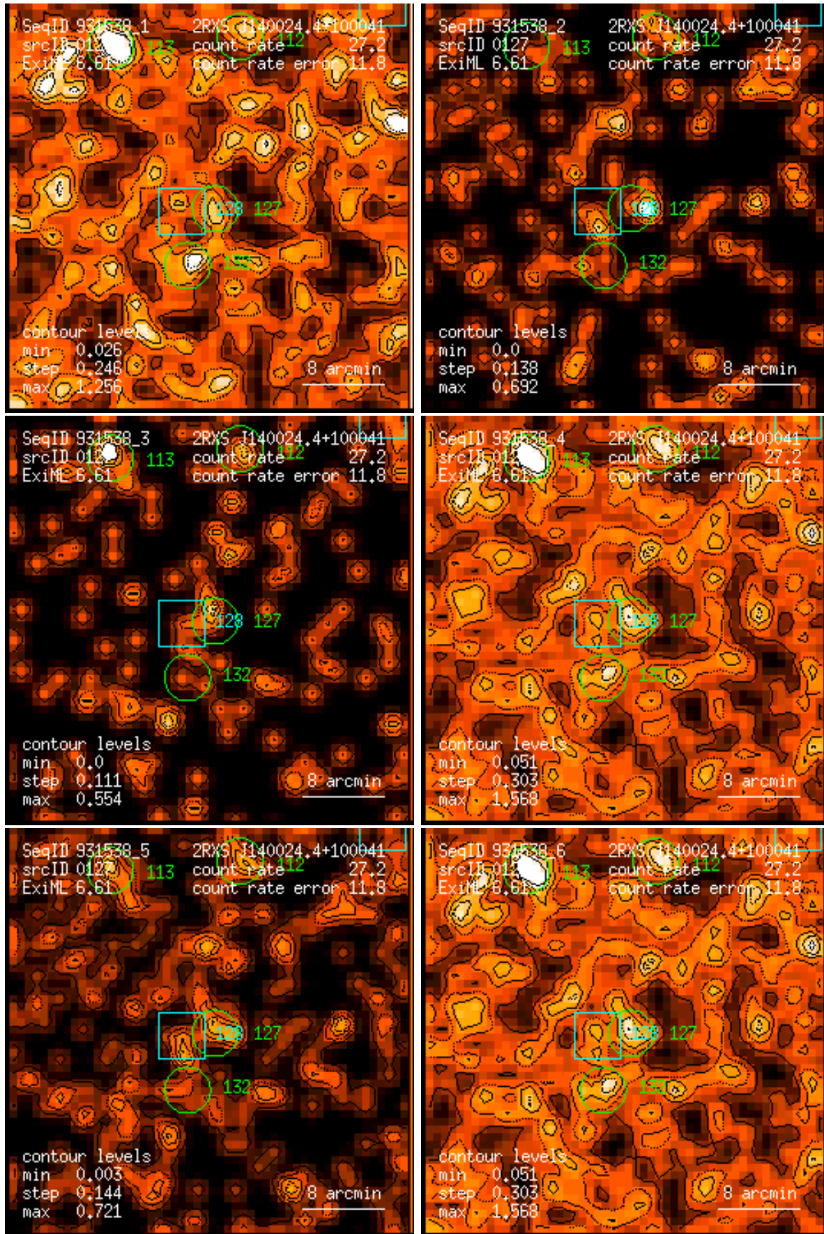
Figure 127: RASS 931538: detection 0127: band rate images, Gaussian filter: (1) PSPC channels 11 – 41, (2) 52 – 90, (3) 91 – 201, (4) 11 – 235, (5) 52 – 201, (6) 11 – 201. Broad band rates in counts/ks. Band rate contour levels in counts/ks/arcmin 2 .
