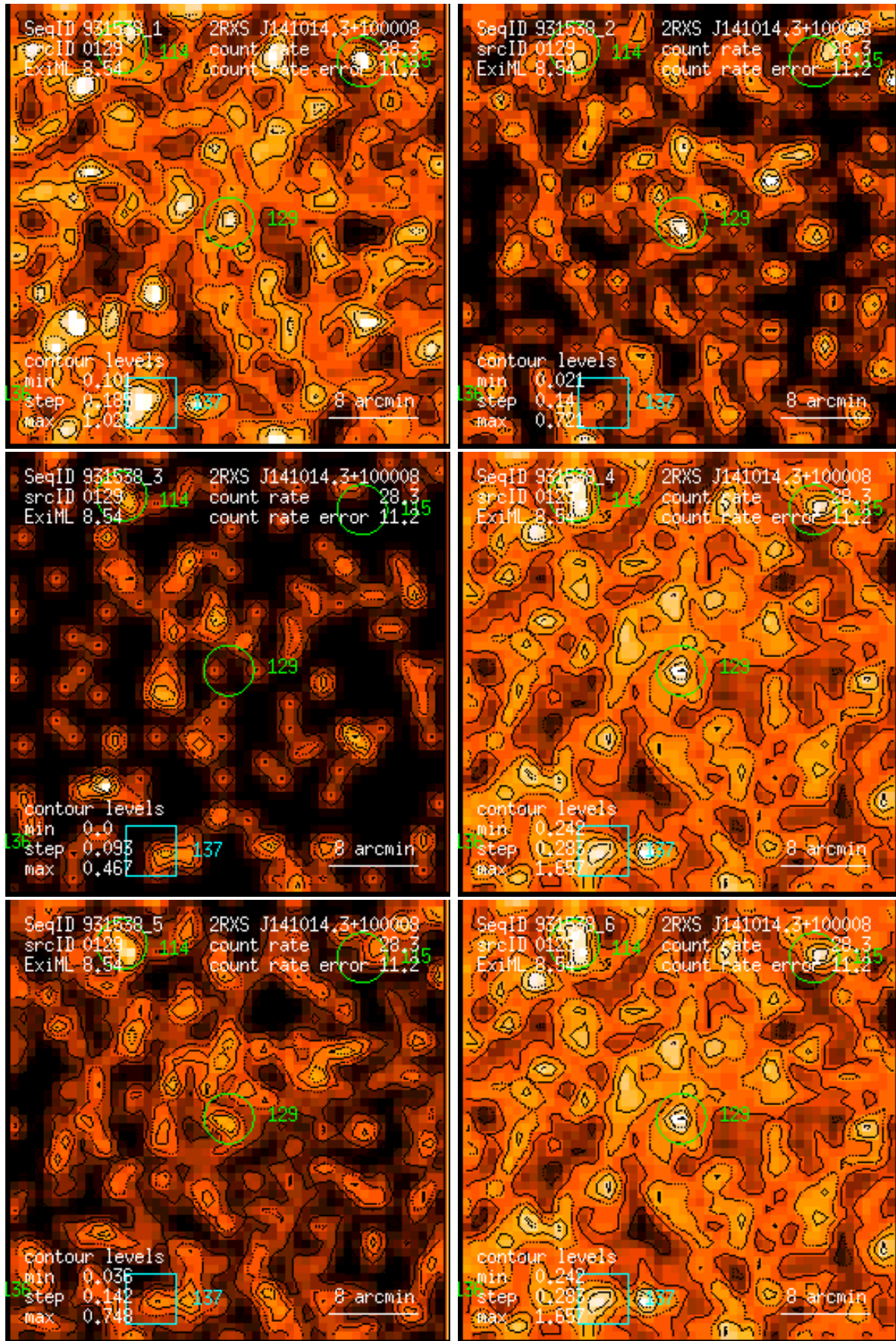
Figure 129: RASS 931538: detection 0129: band rate images, Gaussian filter: (1) PSPC channels 11 – 41, (2) 52 – 90, (3) 91 – 201, (4) 11 – 235, (5) 52 – 201, (6) 11 – 201. Broad band rates in counts/ks. Band rate contour levels in counts/ks/arcmin 2 .
