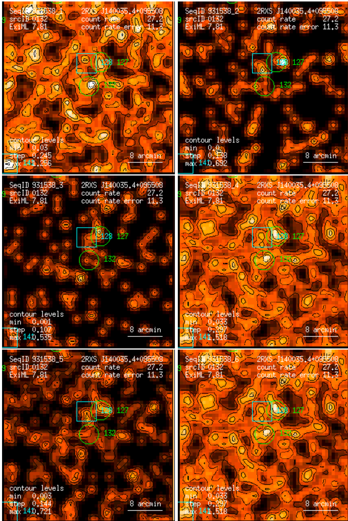
Figure 132: RASS 931538: detection 0132: band rate images, Gaussian filter: (1) PSPC channels 11 – 41, (2) 52 – 90, (3) 91 – 201, (4) 11 – 235, (5) 52 – 201, (6) 11 – 201. Broad band rates in counts/ks. Band rate contour levels in counts/ks/arcmin 2 .
