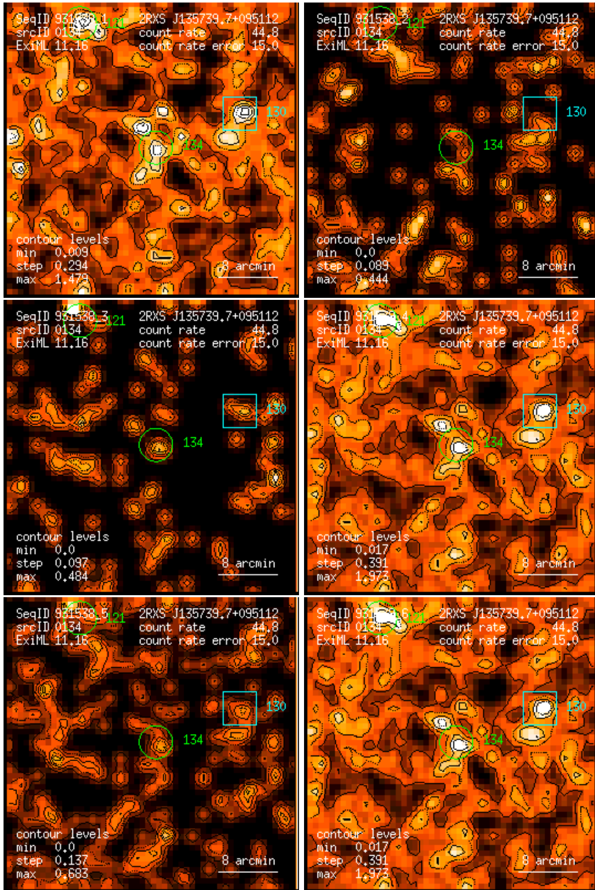
Figure 134: RASS 931538: detection 0134: band rate images, Gaussian filter: (1) PSPC channels 11 – 41, (2) 52 – 90, (3) 91 – 201, (4) 11 – 235, (5) 52 – 201, (6) 11 – 201. Broad band rates in counts/ks. Band rate contour levels in counts/ks/arcmin 2 .
