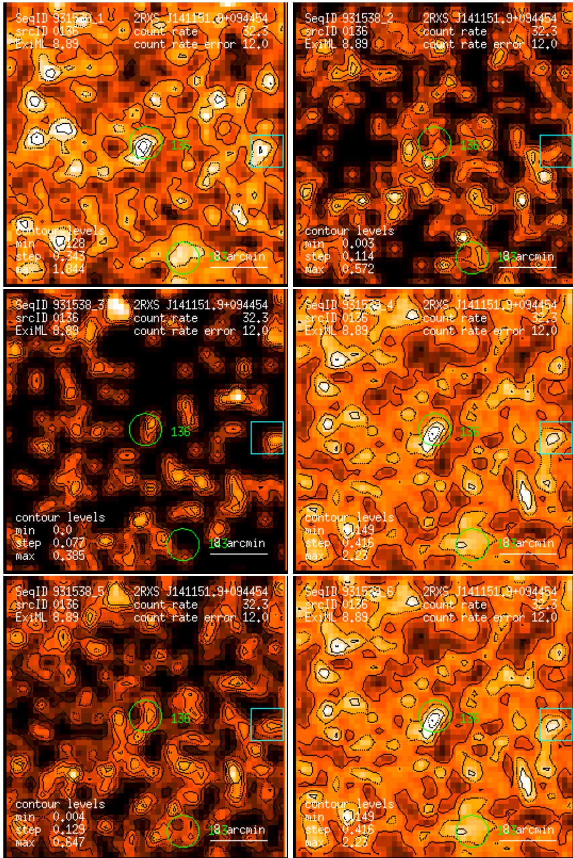
Figure 136: RASS 931538: detection 0136: band rate images, Gaussian filter: (1) PSPC channels 11 – 41, (2) 52 – 90, (3) 91 – 201, (4) 11 – 235, (5) 52 – 201, (6) 11 – 201. Broad band rates in counts/ks. Band rate contour levels in counts/ks/arcmin 2 .
