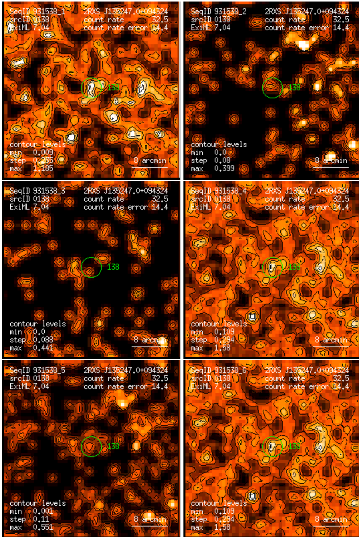
Figure 138: RASS 931538: detection 0138: band rate images, Gaussian filter: (1) PSPC channels 11 – 41, (2) 52 – 90, (3) 91 – 201, (4) 11 – 235, (5) 52 – 201, (6) 11 – 201. Broad band rates in counts/ks. Band rate contour levels in counts/ks/arcmin 2 .
