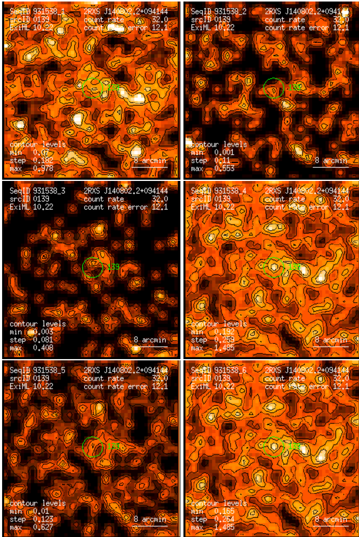
Figure 139: RASS 931538: detection 0139: band rate images, Gaussian filter: (1) PSPC channels 11 – 41, (2) 52 – 90, (3) 91 – 201, (4) 11 – 235, (5) 52 – 201, (6) 11 – 201. Broad band rates in counts/ks. Band rate contour levels in counts/ks/arcmin 2 .
