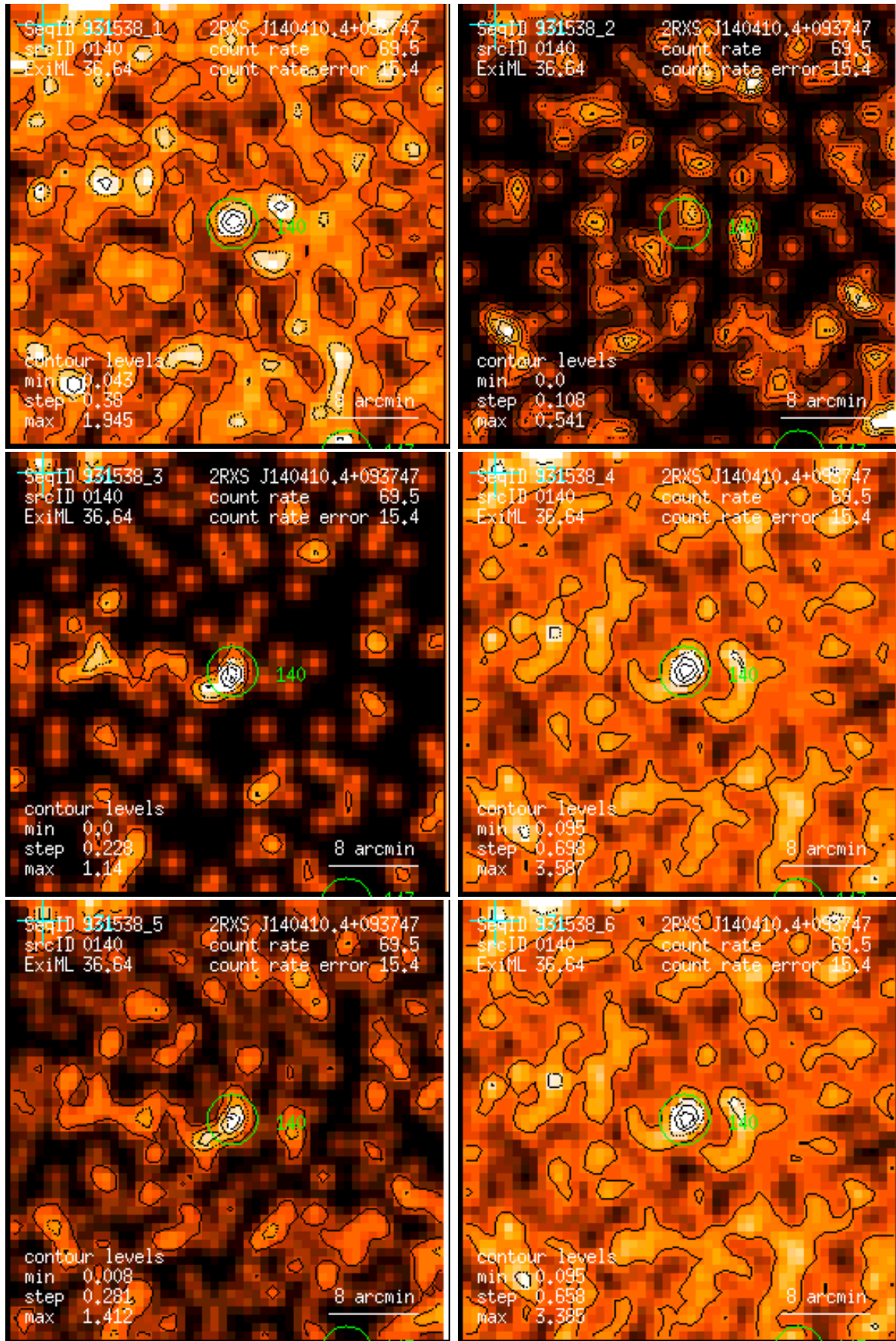
Figure 140: RASS 931538: detection 0140: band rate images, Gaussian filter: (1) PSPC channels 11 – 41, (2) 52 – 90, (3) 91 – 201, (4) 11 – 235, (5) 52 – 201, (6) 11 – 201. Broad band rates in counts/ks. Band rate contour levels in counts/ks/arcmin 2 .
