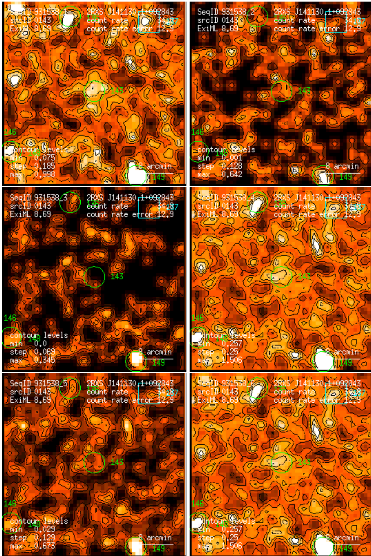
Figure 143: RASS 931538: detection 0143: band rate images, Gaussian filter: (1) PSPC channels 11 – 41, (2) 52 – 90, (3) 91 – 201, (4) 11 – 235, (5) 52 – 201, (6) 11 – 201. Broad band rates in counts/ks. Band rate contour levels in counts/ks/arcmin 2 .
