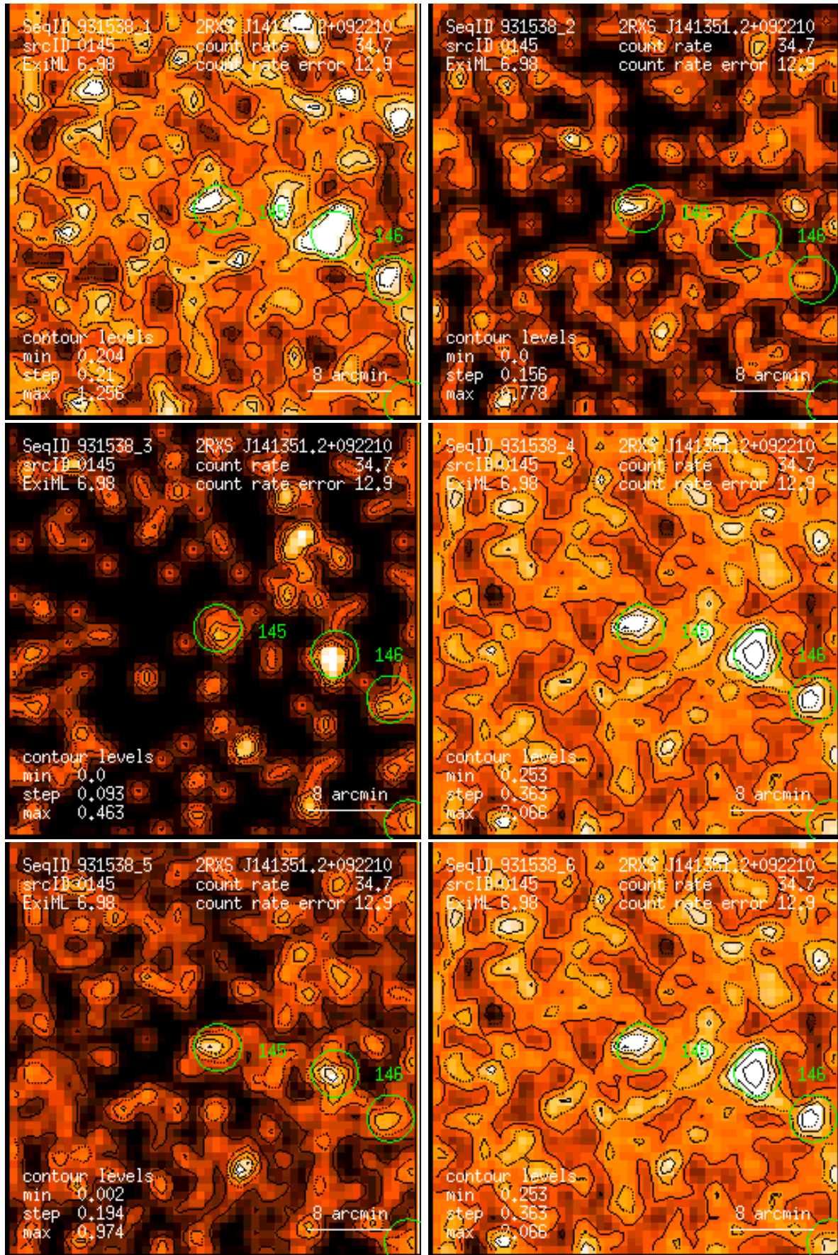
Figure 145: RASS 931538: detection 0145: band rate images, Gaussian filter: (1) PSPC channels 11 – 41, (2) 52 – 90, (3) 91 – 201, (4) 11 – 235, (5) 52 – 201, (6) 11 – 201. Broad band rates in counts/ks. Band rate contour levels in counts/ks/arcmin 2 .
