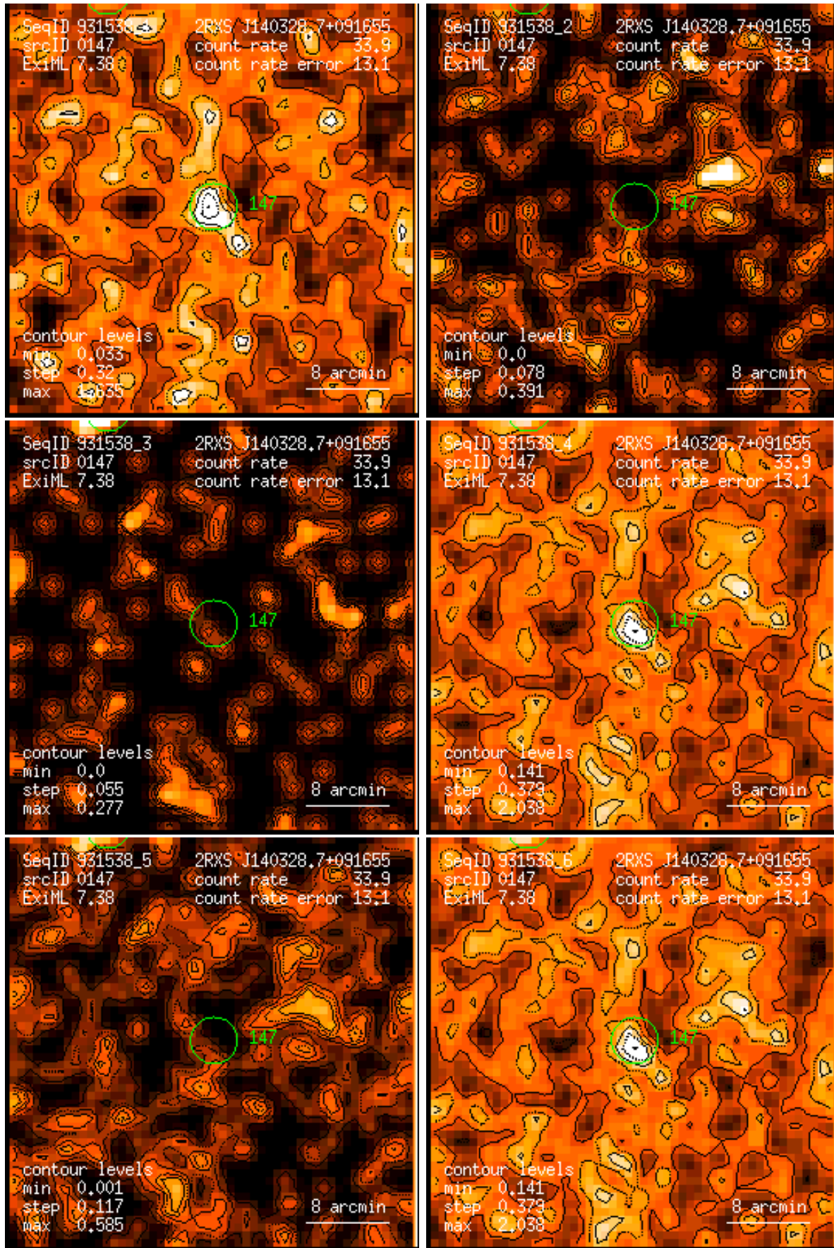
Figure 147: RASS 931538: detection 0147: band rate images, Gaussian filter: (1) PSPC channels 11 – 41, (2) 52 – 90, (3) 91 – 201, (4) 11 – 235, (5) 52 – 201, (6) 11 – 201. Broad band rates in counts/ks. Band rate contour levels in counts/ks/arcmin 2 .
