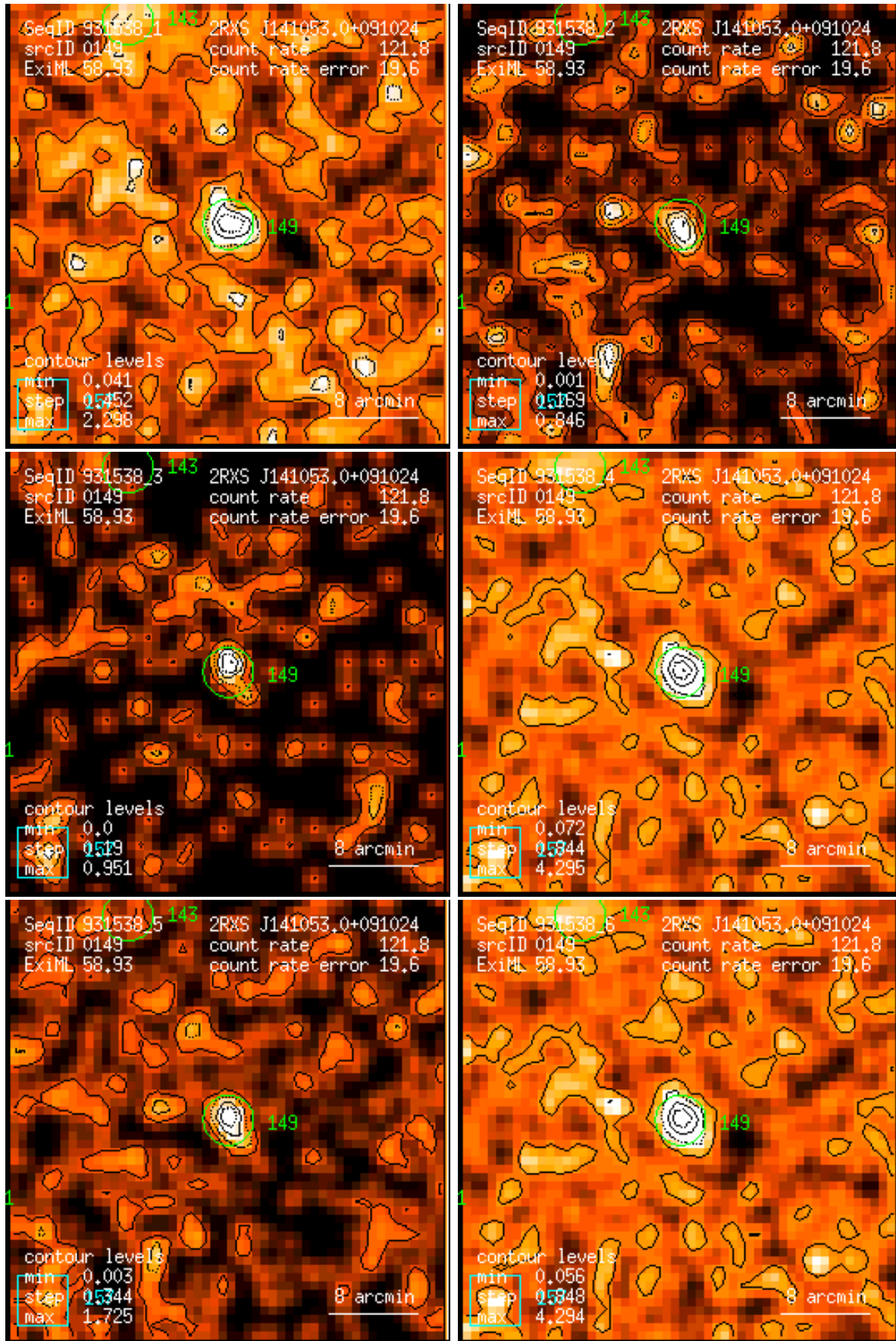
Figure 149: RASS 931538: detection 0149: band rate images, Gaussian filter: (1) PSPC channels 11 – 41, (2) 52 – 90, (3) 91 – 201, (4) 11 – 235, (5) 52 – 201, (6) 11 – 201. Broad band rates in counts/ks. Band rate contour levels in counts/ks/arcmin 2 .
