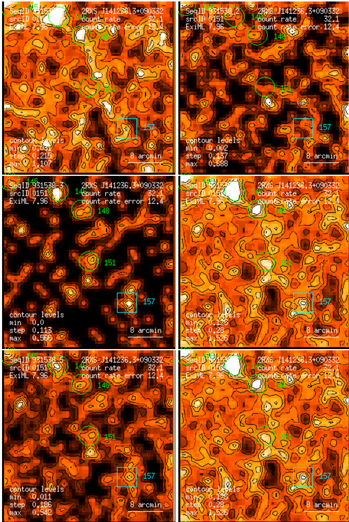
Figure 151: RASS 931538: detection 0151: band rate images, Gaussian filter: (1) PSPC channels 11 – 41, (2) 52 – 90, (3) 91 – 201, (4) 11 – 235, (5) 52 – 201, (6) 11 – 201. Broad band rates in counts/ks. Band rate contour levels in counts/ks/arcmin 2 .
