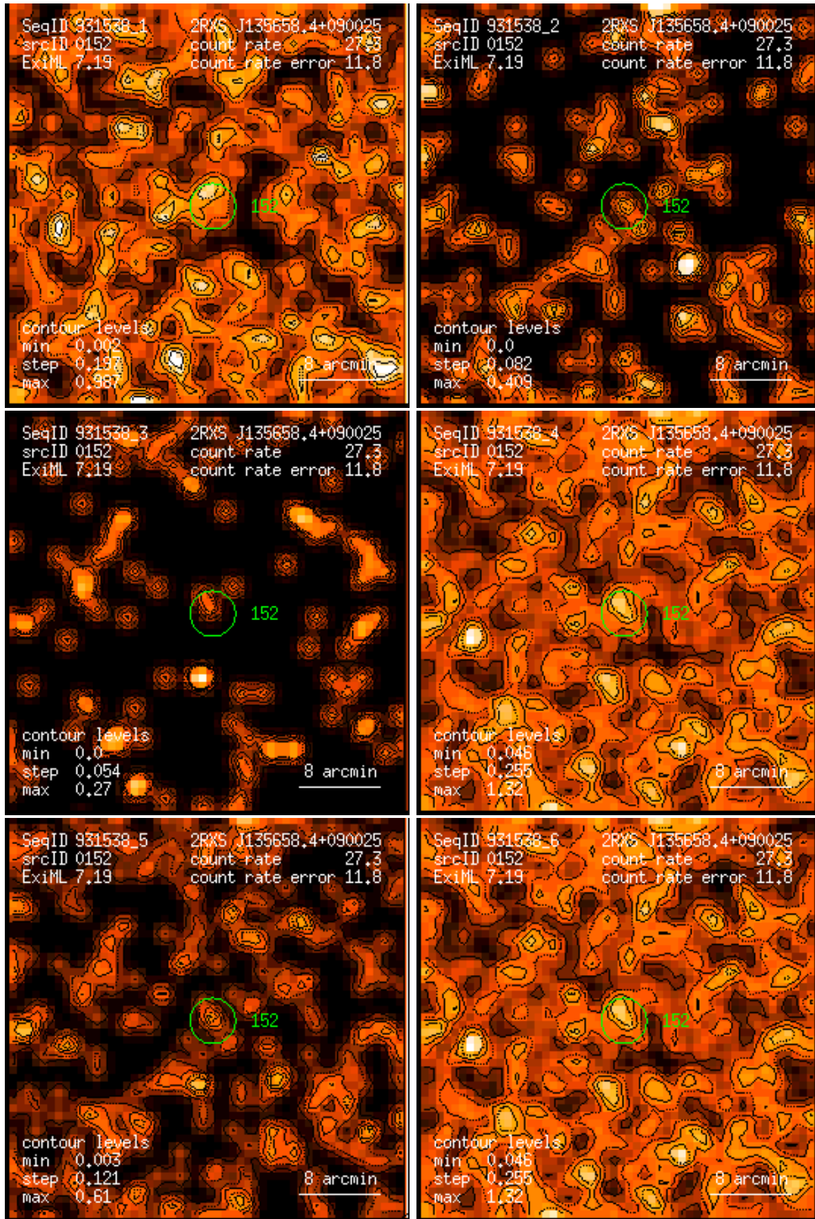
Figure 152: RASS 931538: detection 0152: band rate images, Gaussian filter: (1) PSPC channels 11 – 41, (2) 52 – 90, (3) 91 – 201, (4) 11 – 235, (5) 52 – 201, (6) 11 – 201. Broad band rates in counts/ks. Band rate contour levels in counts/ks/arcmin 2 .
