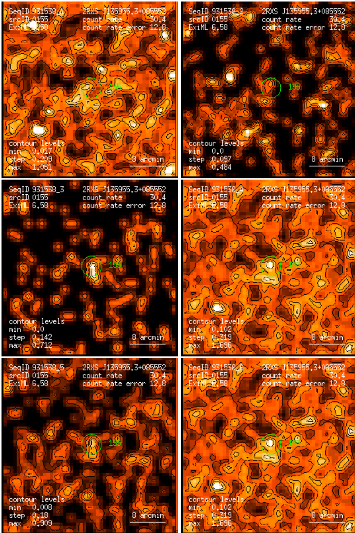
Figure 155: RASS 931538: detection 0155: band rate images, Gaussian filter: (1) PSPC channels 11 – 41, (2) 52 – 90, (3) 91 – 201, (4) 11 – 235, (5) 52 – 201, (6) 11 – 201. Broad band rates in counts/ks. Band rate contour levels in counts/ks/arcmin 2 .
