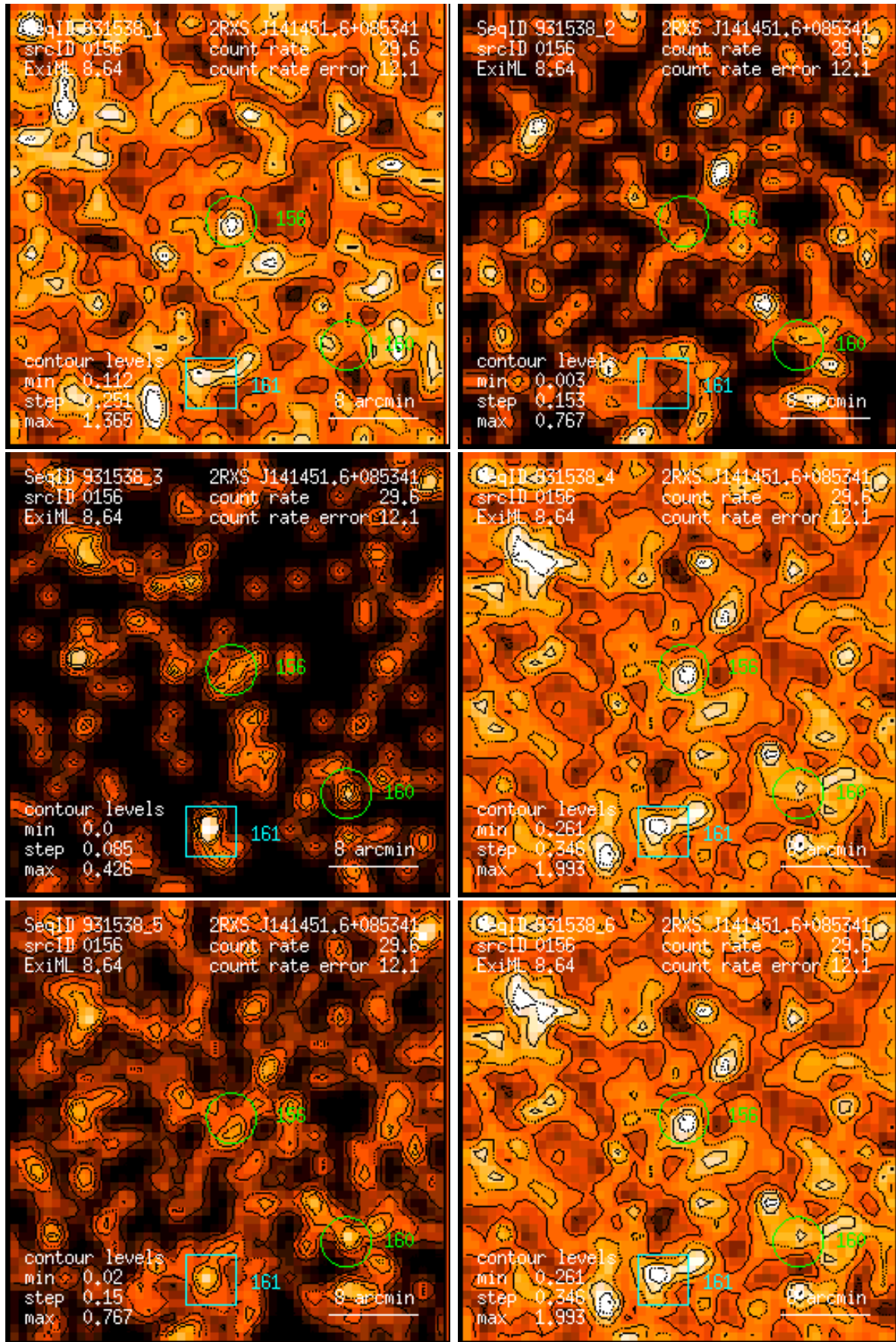
Figure 156: RASS 931538: detection 0156: band rate images, Gaussian filter: (1) PSPC channels 11 – 41, (2) 52 – 90, (3) 91 – 201, (4) 11 – 235, (5) 52 – 201, (6) 11 – 201. Broad band rates in counts/ks. Band rate contour levels in counts/ks/arcmin 2 .
