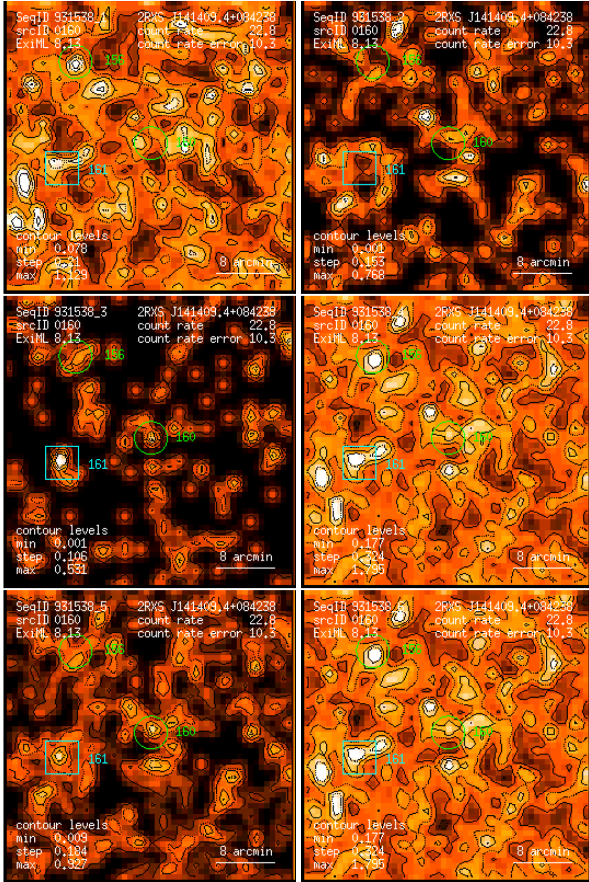
Figure 160: RASS 931538: detection 0160: band rate images, Gaussian filter: (1) PSPC channels 11 – 41, (2) 52 – 90, (3) 91 – 201, (4) 11 – 235, (5) 52 – 201, (6) 11 – 201. Broad band rates in counts/ks. Band rate contour levels in counts/ks/arcmin 2 .
