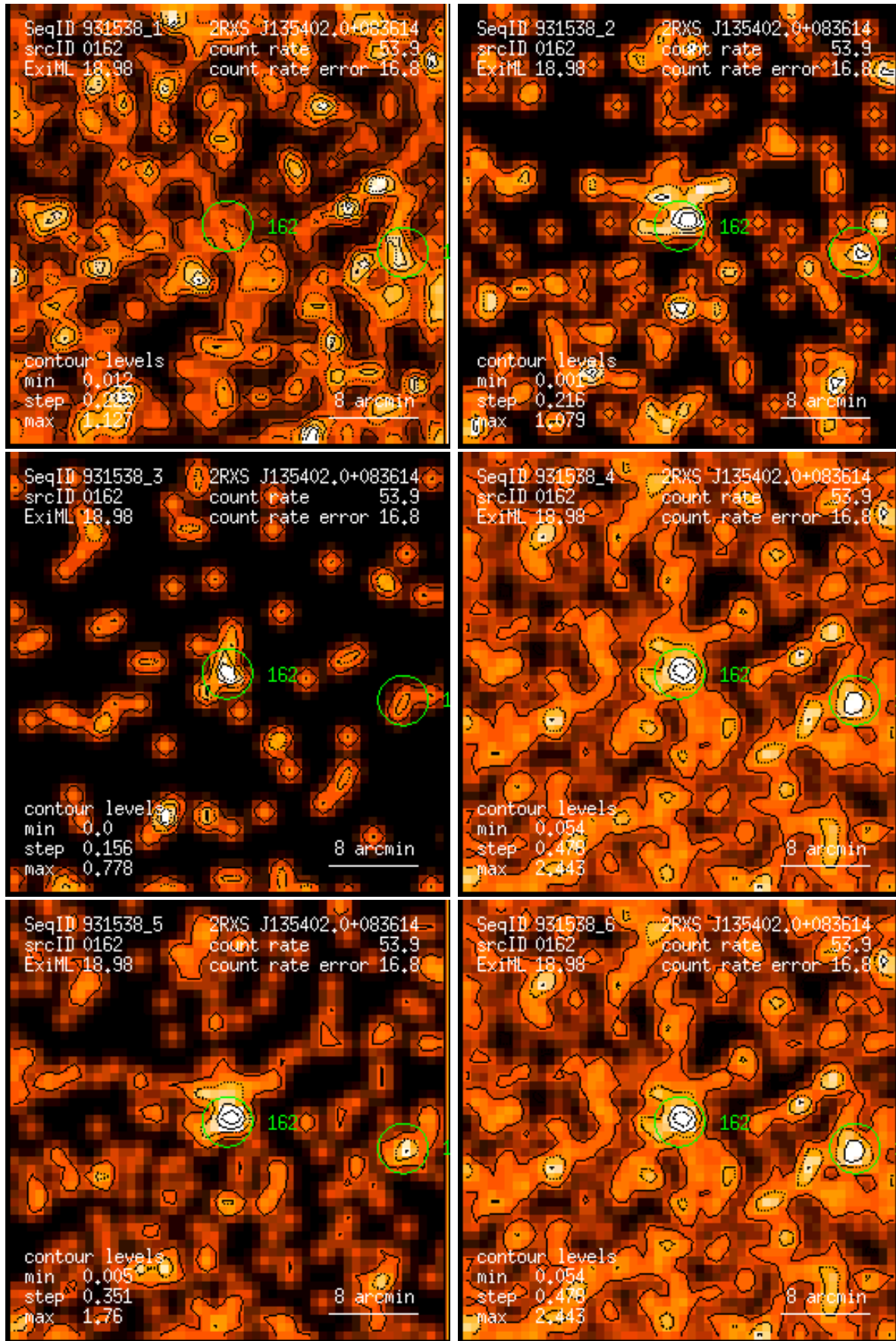
Figure 162: RASS 931538: detection 0162: band rate images, Gaussian filter: (1) PSPC channels 11 – 41, (2) 52 – 90, (3) 91 – 201, (4) 11 – 235, (5) 52 – 201, (6) 11 – 201. Broad band rates in counts/ks. Band rate contour levels in counts/ks/arcmin 2 .
