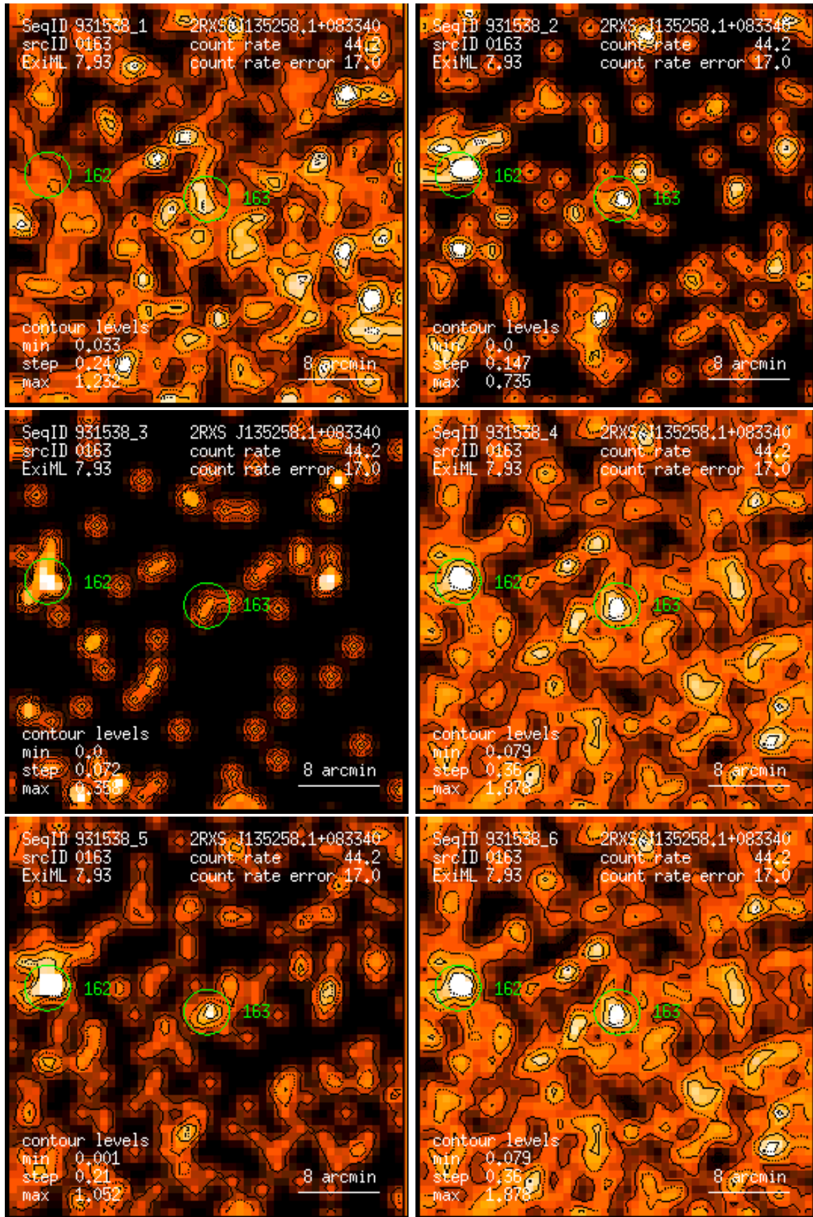
Figure 163: RASS 931538: detection 0163: band rate images, Gaussian filter: (1) PSPC channels 11 – 41, (2) 52 – 90, (3) 91 – 201, (4) 11 – 235, (5) 52 – 201, (6) 11 – 201. Broad band rates in counts/ks. Band rate contour levels in counts/ks/arcmin 2 .
