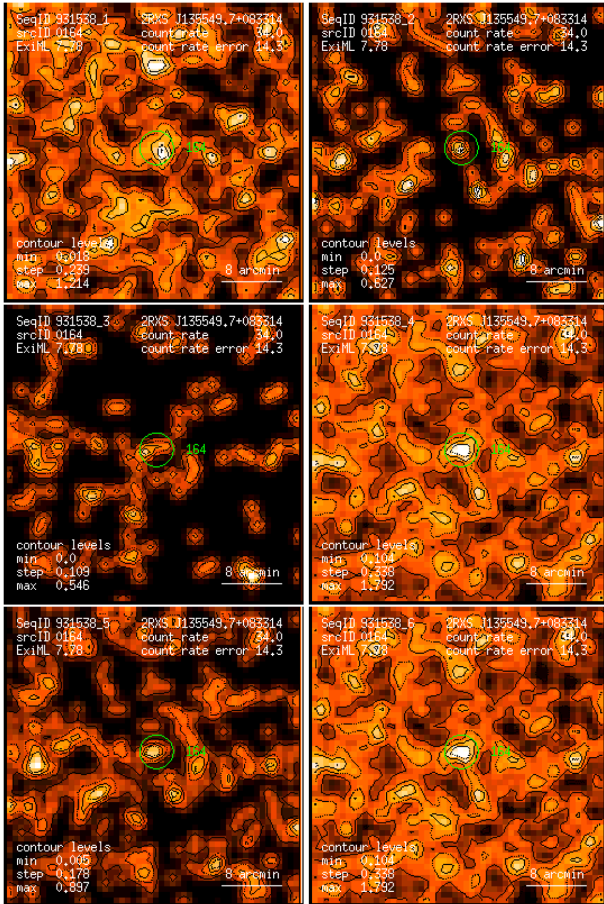
Figure 164: RASS 931538: detection 0164: band rate images, Gaussian filter: (1) PSPC channels 11 – 41, (2) 52 – 90, (3) 91 – 201, (4) 11 – 235, (5) 52 – 201, (6) 11 – 201. Broad band rates in counts/ks. Band rate contour levels in counts/ks/arcmin 2 .
