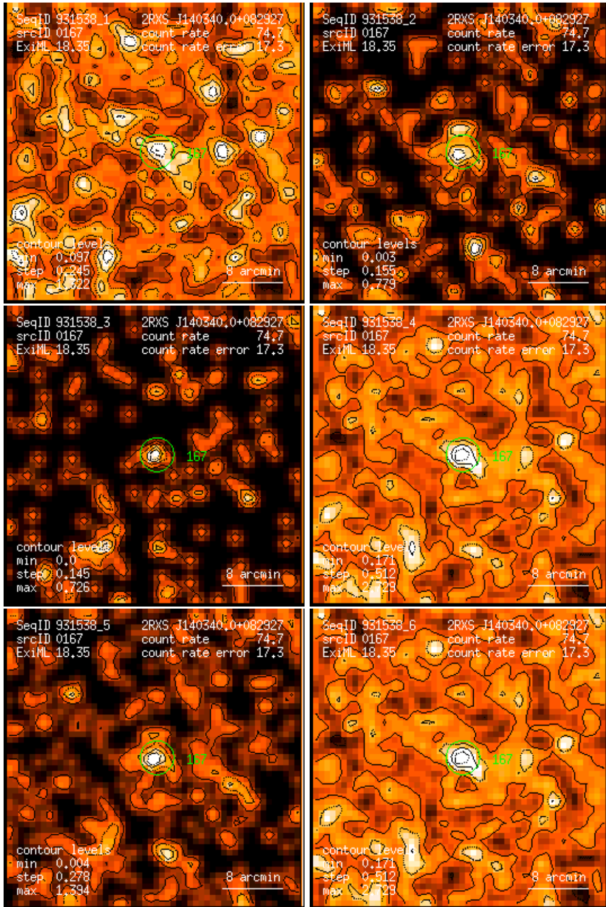
Figure 167: RASS 931538: detection 0167: band rate images, Gaussian filter: (1) PSPC channels 11 – 41, (2) 52 – 90, (3) 91 – 201, (4) 11 – 235, (5) 52 – 201, (6) 11 – 201. Broad band rates in counts/ks. Band rate contour levels in counts/ks/arcmin 2 .
