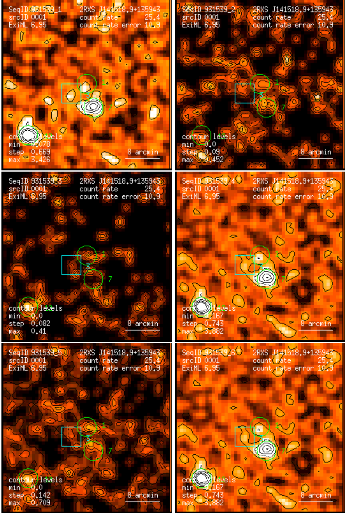
Figure 1: RASS 931539: detection 0001: band rate images, Gaussian filter: (1) PSPC channels 11 – 41, (2) 52 – 90, (3) 91 – 201, (4) 11 – 235, (5) 52 – 201, (6) 11 – 201. Broad band rates in counts/ks. Band rate contour levels in counts/ks/arcmin 2 .
