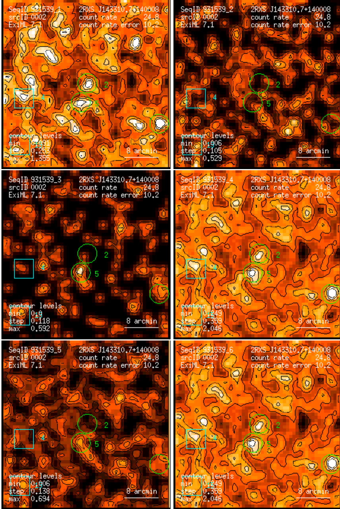
Figure 2: RASS 931539: detection 0002: band rate images, Gaussian filter: (1) PSPC channels 11 – 41, (2) 52 – 90, (3) 91 – 201, (4) 11 – 235, (5) 52 – 201, (6) 11 – 201. Broad band rates in counts/ks. Band rate contour levels in counts/ks/arcmin 2 .
