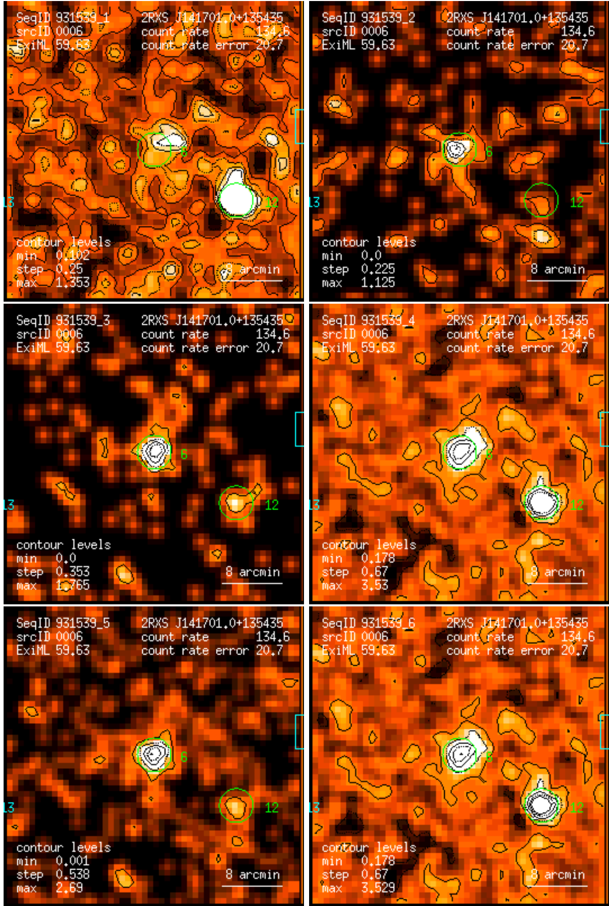
Figure 6: RASS 931539: detection 0006: band rate images, Gaussian filter: (1) PSPC channels 11 – 41, (2) 52 – 90, (3) 91 – 201, (4) 11 – 235, (5) 52 – 201, (6) 11 – 201. Broad band rates in counts/ks. Band rate contour levels in counts/ks/arcmin 2 .
