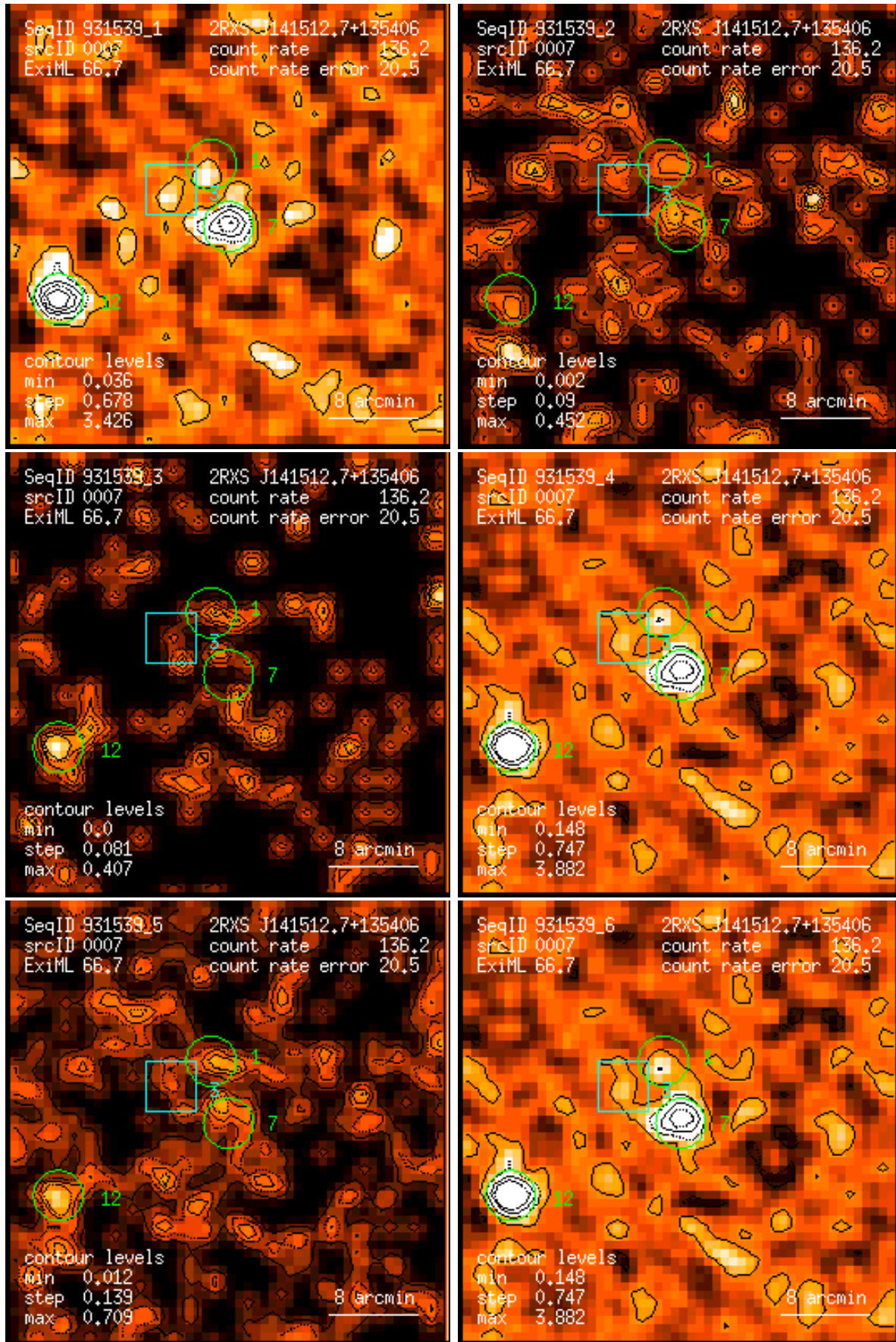
Figure 7: RASS 931539: detection 0007: band rate images, Gaussian filter: (1) PSPC channels 11 – 41, (2) 52 – 90, (3) 91 – 201, (4) 11 – 235, (5) 52 – 201, (6) 11 – 201. Broad band rates in counts/ks. Band rate contour levels in counts/ks/arcmin 2 .
