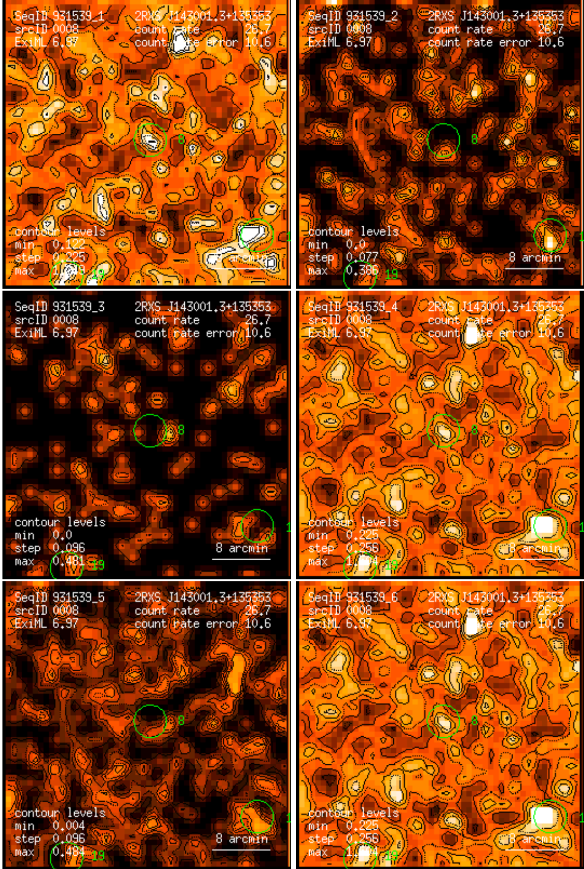
Figure 8: RASS 931539: detection 0008: band rate images, Gaussian filter: (1) PSPC channels 11 – 41, (2) 52 – 90, (3) 91 – 201, (4) 11 – 235, (5) 52 – 201, (6) 11 – 201. Broad band rates in counts/ks. Band rate contour levels in counts/ks/arcmin 2 .
