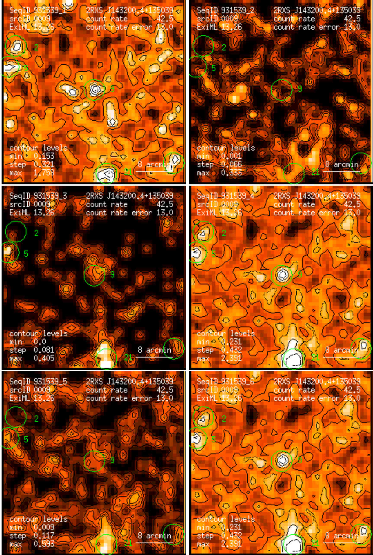
Figure 9: RASS 931539: detection 0009: band rate images, Gaussian filter: (1) PSPC channels 11 – 41, (2) 52 – 90, (3) 91 – 201, (4) 11 – 235, (5) 52 – 201, (6) 11 – 201. Broad band rates in counts/ks. Band rate contour levels in counts/ks/arcmin 2 .
