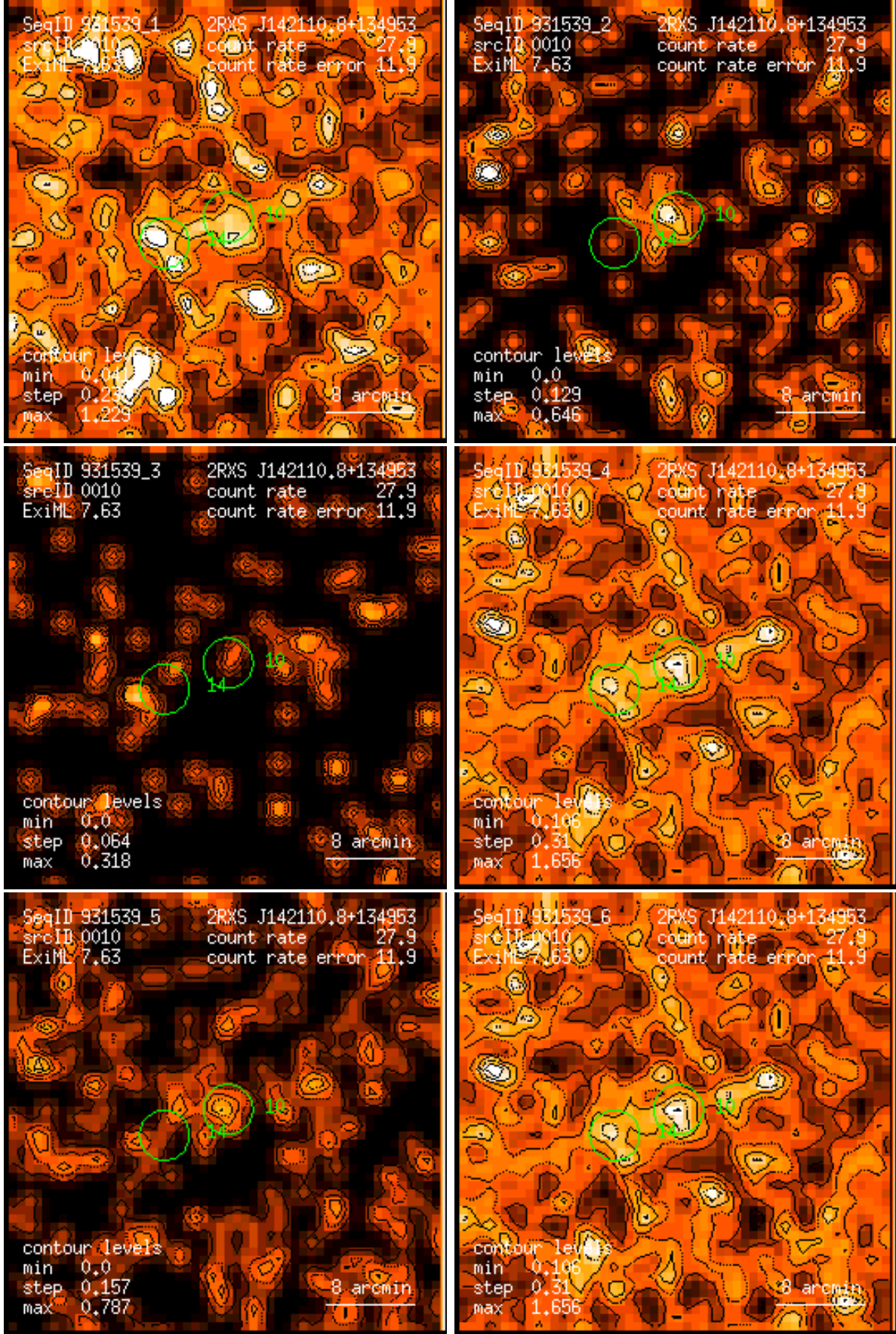
Figure 10: RASS 931539: detection 0010: band rate images, Gaussian filter: (1) PSPC channels 11 – 41, (2) 52 – 90, (3) 91 – 201, (4) 11 – 235, (5) 52 – 201, (6) 11 – 201. Broad band rates in counts/ks. Band rate contour levels in counts/ks/arcmin 2 .
