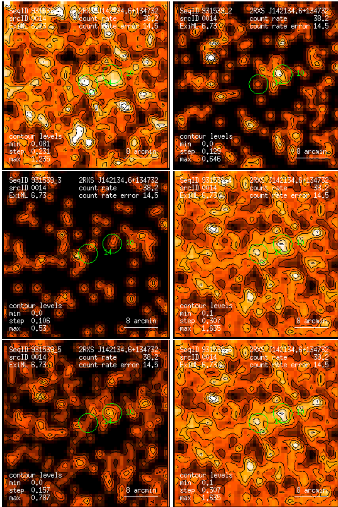
Figure 14: RASS 931539: detection 0014: band rate images, Gaussian filter: (1) PSPC channels 11 – 41, (2) 52 – 90, (3) 91 – 201, (4) 11 – 235, (5) 52 – 201, (6) 11 – 201. Broad band rates in counts/ks. Band rate contour levels in counts/ks/arcmin 2 .
