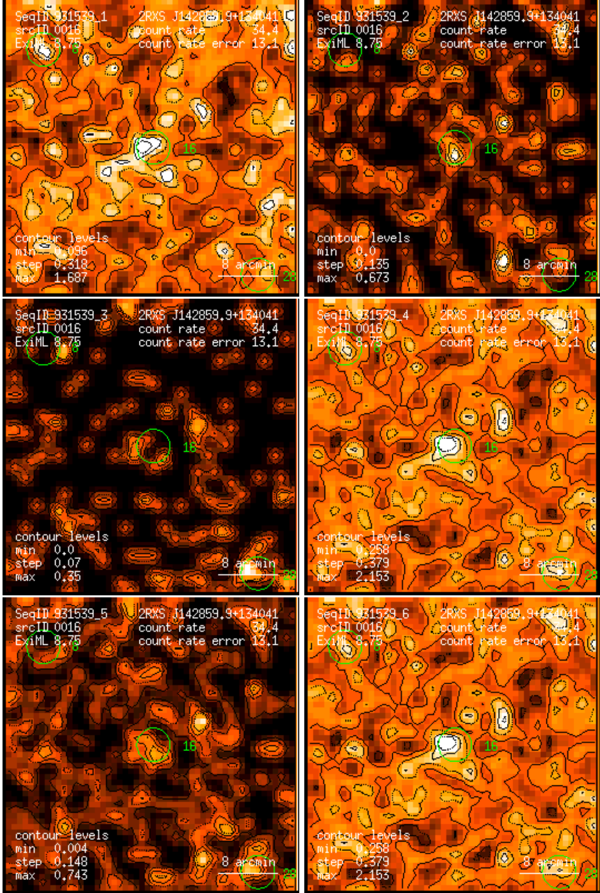
Figure 16: RASS 931539: detection 0016: band rate images, Gaussian filter: (1) PSPC channels 11 – 41, (2) 52 – 90, (3) 91 – 201, (4) 11 – 235, (5) 52 – 201, (6) 11 – 201. Broad band rates in counts/ks. Band rate contour levels in counts/ks/arcmin 2 .
