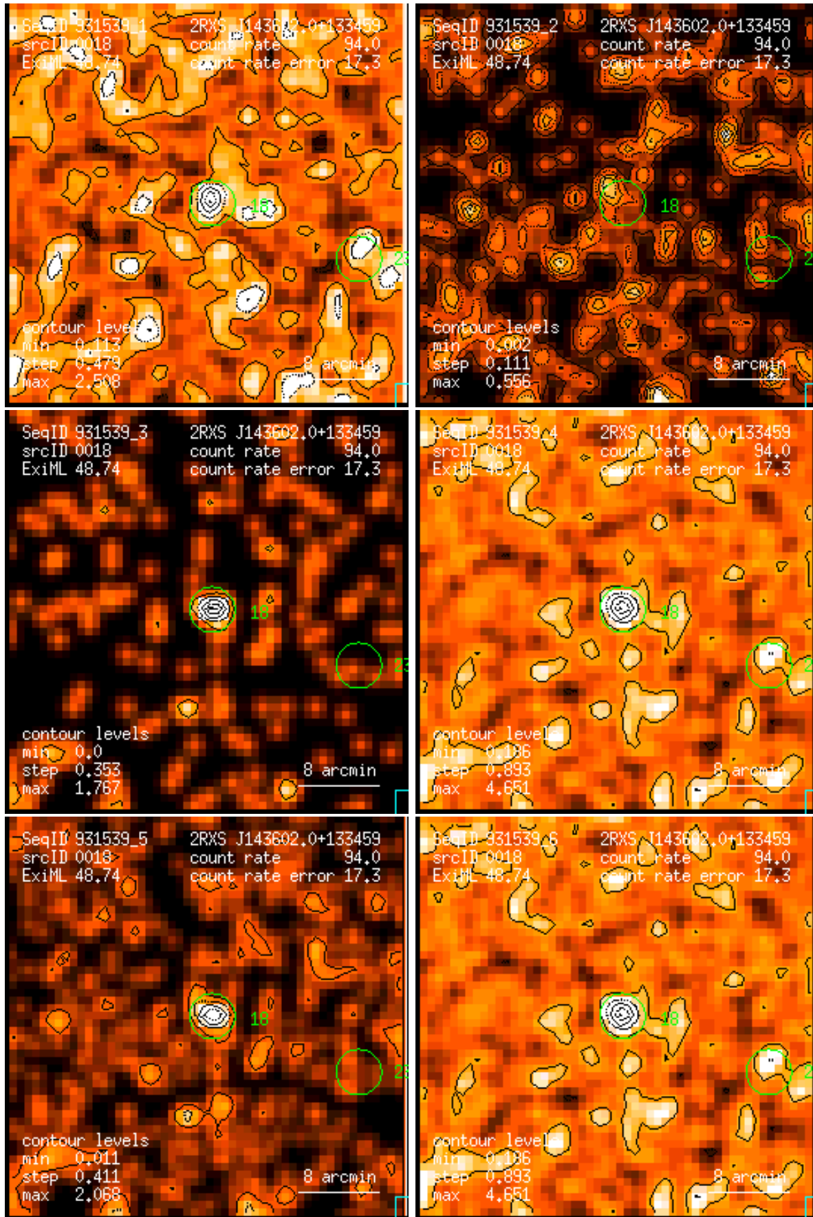
Figure 18: RASS 931539: detection 0018: band rate images, Gaussian filter: (1) PSPC channels 11 – 41, (2) 52 – 90, (3) 91 – 201, (4) 11 – 235, (5) 52 – 201, (6) 11 – 201. Broad band rates in counts/ks. Band rate contour levels in counts/ks/arcmin 2 .
