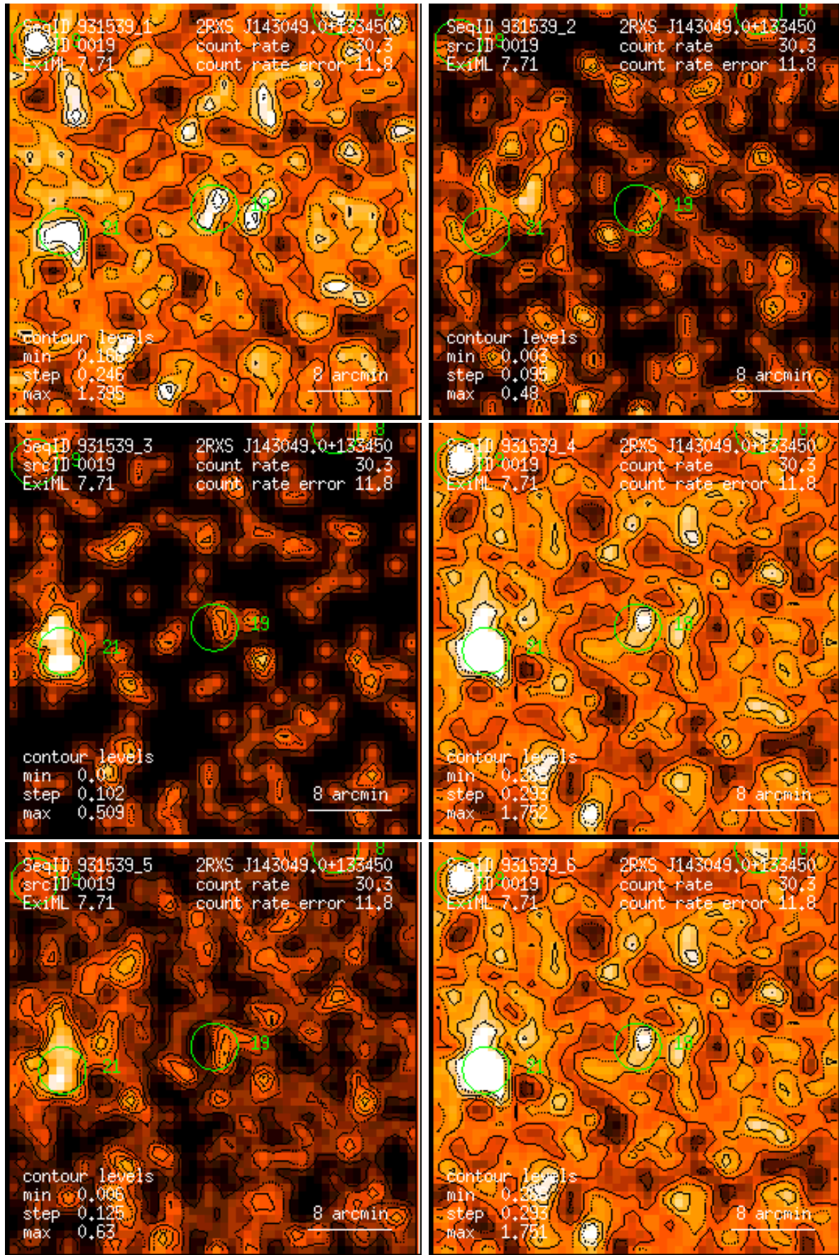
Figure 19: RASS 931539: detection 0019: band rate images, Gaussian filter: (1) PSPC channels 11 – 41, (2) 52 – 90, (3) 91 – 201, (4) 11 – 235, (5) 52 – 201, (6) 11 – 201. Broad band rates in counts/ks. Band rate contour levels in counts/ks/arcmin 2 .
