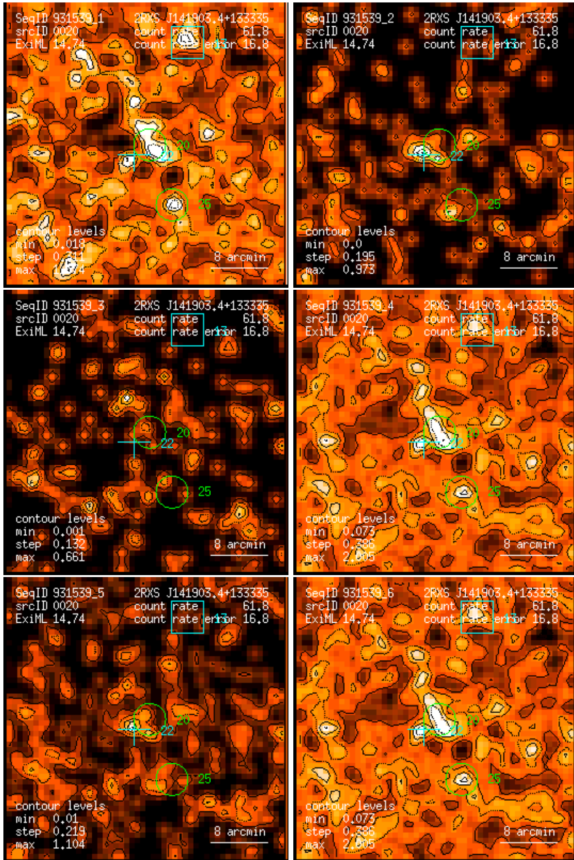
Figure 20: RASS 931539: detection 0020: band rate images, Gaussian filter: (1) PSPC channels 11 – 41, (2) 52 – 90, (3) 91 – 201, (4) 11 – 235, (5) 52 – 201, (6) 11 – 201. Broad band rates in counts/ks. Band rate contour levels in counts/ks/arcmin 2 .
