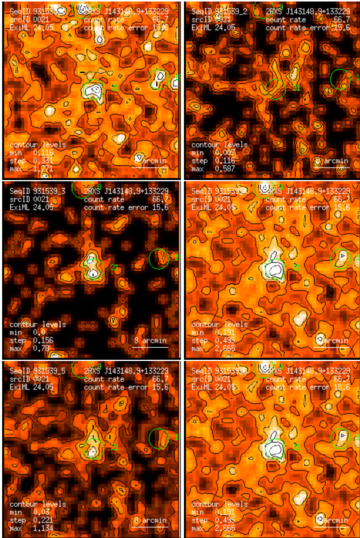
Figure 21: RASS 931539: detection 0021: band rate images, Gaussian filter: (1) PSPC channels 11 – 41, (2) 52 – 90, (3) 91 – 201, (4) 11 – 235, (5) 52 – 201, (6) 11 – 201. Broad band rates in counts/ks. Band rate contour levels in counts/ks/arcmin 2 .
