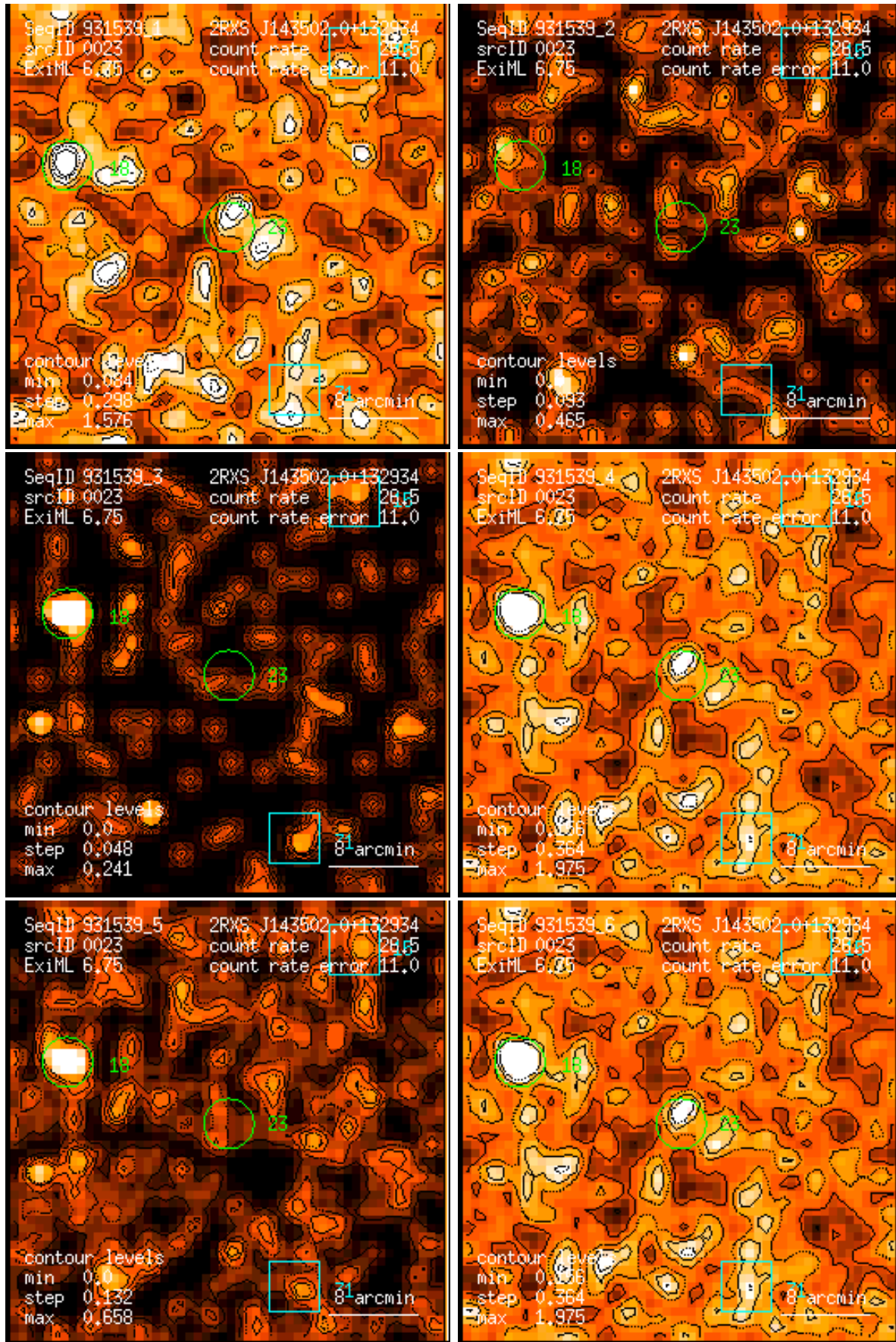
Figure 23: RASS 931539: detection 0023: band rate images, Gaussian filter: (1) PSPC channels 11 – 41, (2) 52 – 90, (3) 91 – 201, (4) 11 – 235, (5) 52 – 201, (6) 11 – 201. Broad band rates in counts/ks. Band rate contour levels in counts/ks/arcmin 2 .
